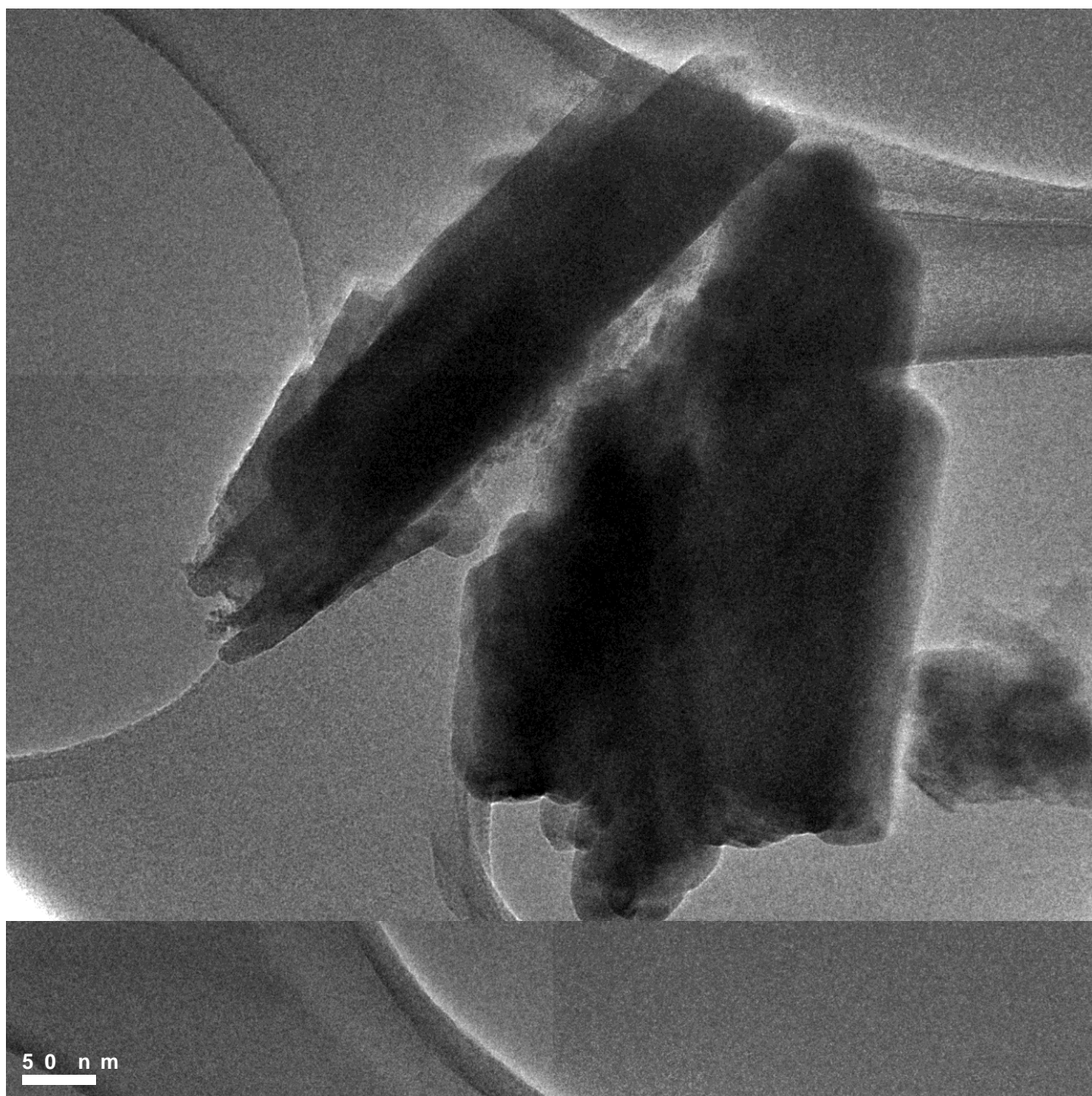
Figure S5. Low magnification TEM image of Fe 2+ -OPAZ sample, showing elongated agglomerates, with sizes of 500 x 130 and 550 x 300 nm.
