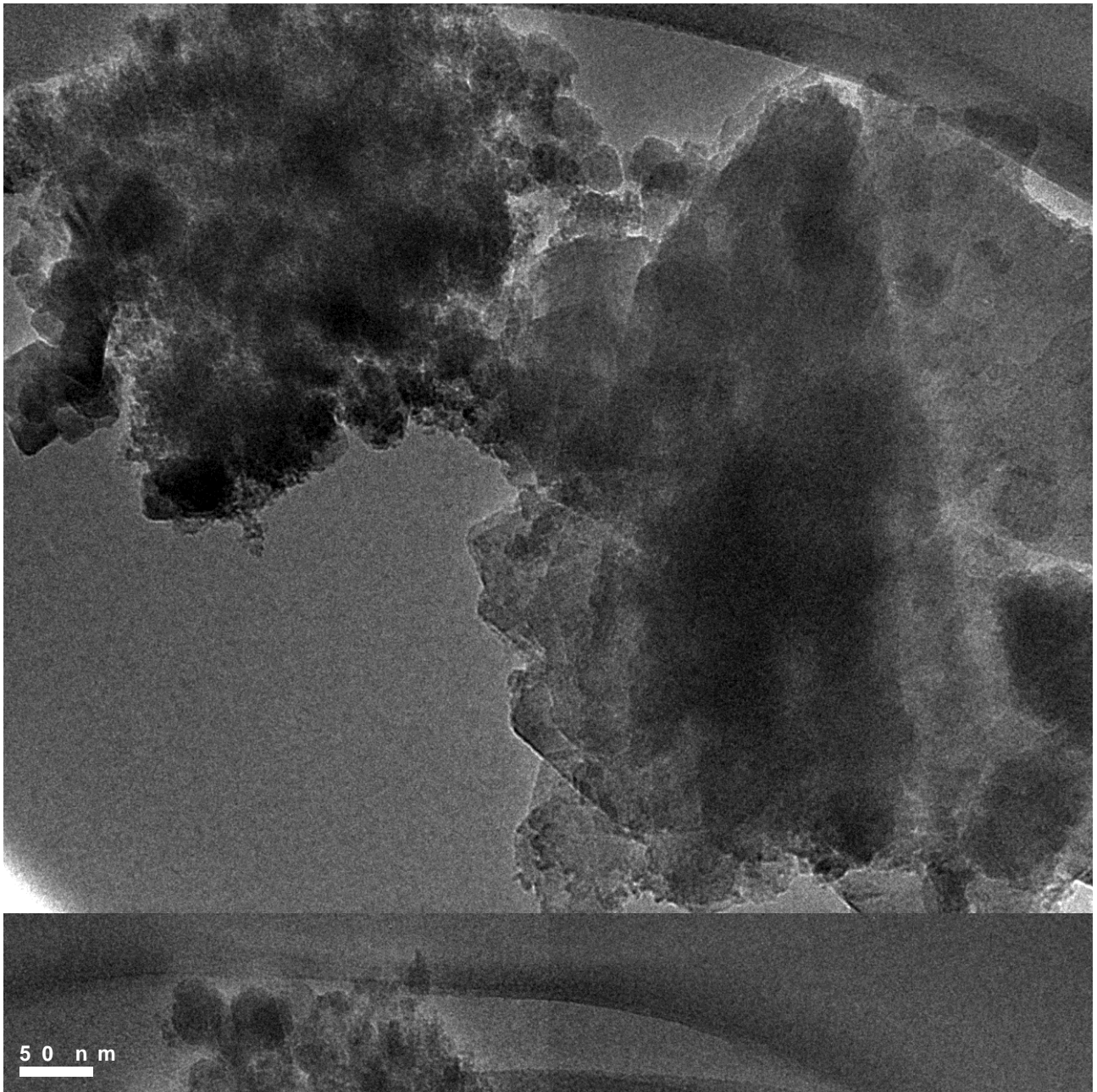
Figure S4. Low magnification TEM image of OPAZ sample, showing large agglomerates covered by an amorphous phase.
