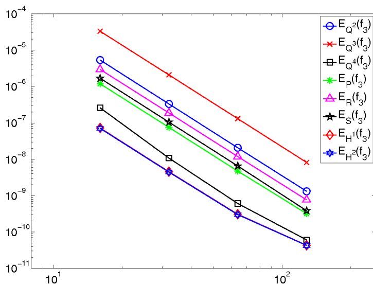
Fig. 4.3 Absolute errors for I(f_3)
