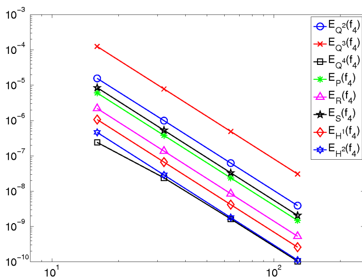
Fig. 4.4 Absolute errors for I(f_4)
