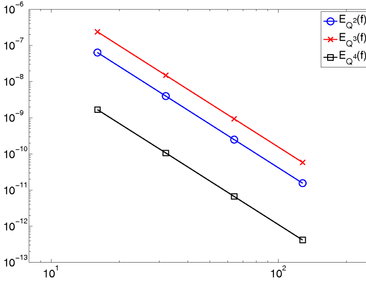
Fig. 4.5 Absolute error for (4.1)
