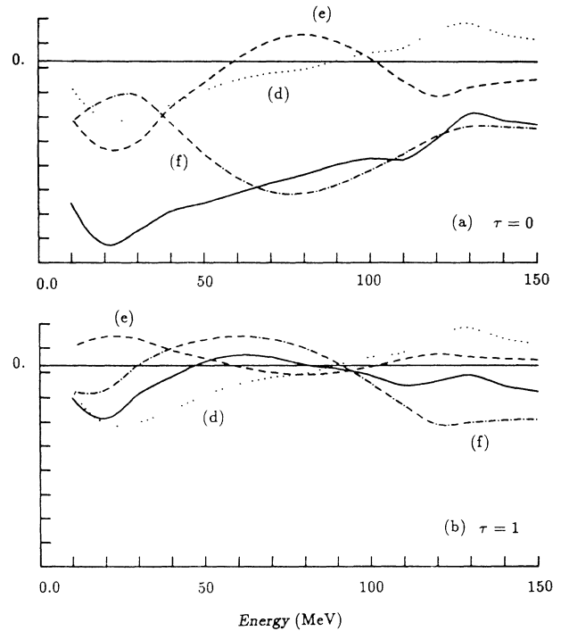
FIG. 3. Separated one-loop contributions in the (a) isoscalar and (b) isovector channels at q = 300 \text{ MeV}/c : The self-energy (dotted line), exchange (dashed line), and correlation (dot-dashed line) contributions are shown. In both channels the solid line is the total.
