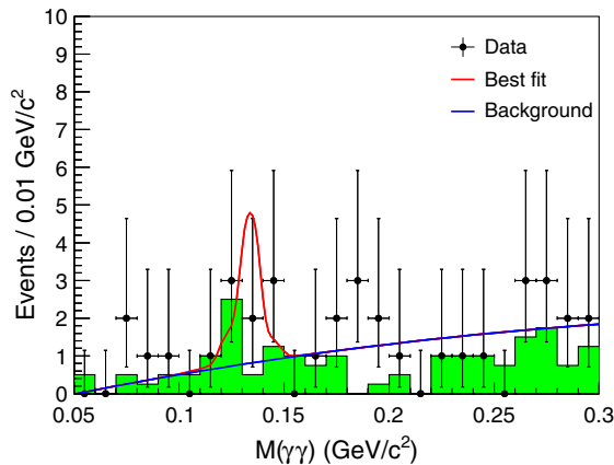
FIG. 3 (color online). Distribution of M(\gamma\gamma) below 0.3 \text{ GeV}/c^2 for J/\psi \rightarrow \mu^+\mu^- . Dots with error bars are data in the J/\psi mass signal region, and the green shaded histogram is from normalized J/\psi mass sideband. The curves show the total fit and the background term.
