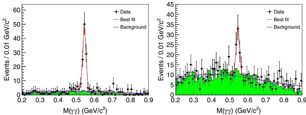
FIG. 2 (color online). Distributions of M(\gamma\gamma) between 0.2 and 0.9 \text{ GeV}/c^2 for J/\psi \rightarrow \mu^+\mu^- (left panel) and for J/\psi \rightarrow e^+e^- (right panel). Dots with error bars are data in the J/\psi mass signal region, and the green shaded histograms are from normalized J/\psi mass sidebands. The curves show the total fit and the background term.
