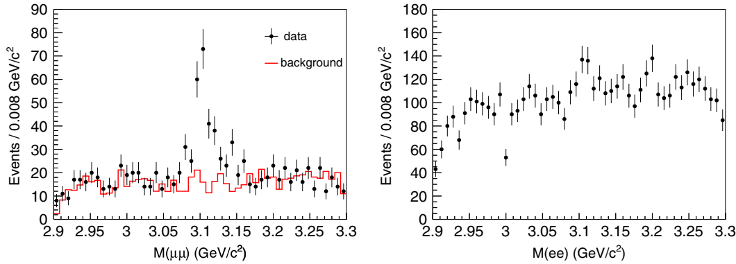
FIG. 1 (color online). (Left panel) M(\mu^+\mu^-) and (right panel) M(e^+e^-) invariant mass distributions. Dots with error bars are data and the open histogram in the left panel shows inclusive-MC-estimated background events.
