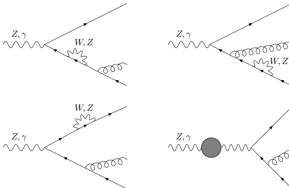
Figure 1: Self-energy insertion graphs. The shaded blob on the incoming wavy line represents all the contributions to the gauge boson self-energy and is dependent on the Higgs mass (hereafter, we will use M_H = 115 \text{ GeV} for the latter). In this and all subsequent figures the graphs in which the exchanged gauge boson is a W -boson is accompanied by corresponding graphs in which the W -boson is replaced by its corresponding Goldstone boson. Since the Yukawa couplings are proportional to the fermion masses, such graphs are only significant in the case of b -quark jets. There is a similar set of diagrams in which the direction of the fermion line is reversed.
