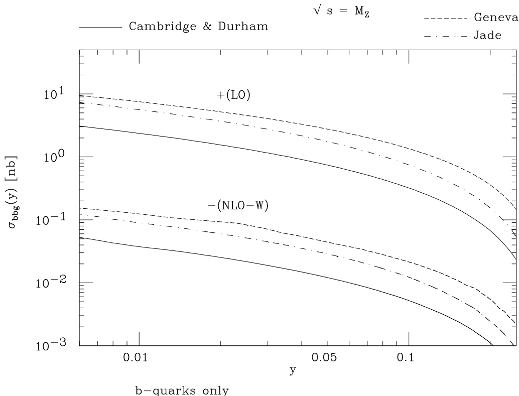
Figure 5: The total cross section for process (4.2) at LO and NLO-W for the Cambridge, Durham, Geneva and Jade jet clustering algorithms, at \sqrt{s} = M_Z . (Notice that the NLO-W results have been plotted with opposite sign for better presentation.)
