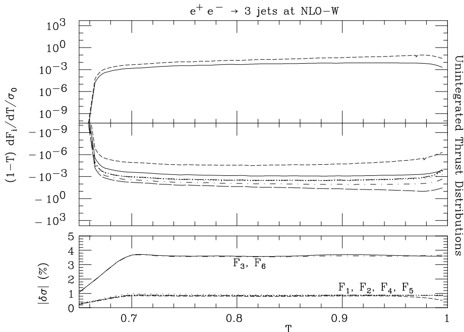
Figure 7: The unintegrated Thrust distributions for the nine component of the cross-section associated to the form-factors in eq. (3.10) for the NLO-W process (4.1) (top and middle) and the relative size of the six components which are non-zero at LO (bottom), at \sqrt{s} = M_Z . Labels are as follows: (top) F_4 (solid), F_3 (short-dashed); (middle) F_9 (solid), F_8 (short-dashed), F_7 (dotted), F_6 (dot-dashed), F_5 (dashed), F_2 (fine-dotted), F_1 (long-dashed); (bottom) F_6 (solid), F_5 (short-dashed), F_4 (dotted), F_3 (dot-dashed), F_2 (dashed), F_1 (fine-dotted).
