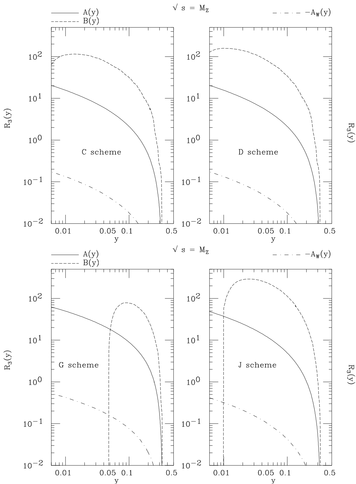
Figure 4: The A(y) , -A_W and B(y) coefficient functions of eqs. (4.4)–(4.5) for the Cambridge, Durham, Geneva and Jade jet clustering algorithms, at \sqrt{s} = M_Z . (Notice that the \sim A_W term has been plotted with opposite sign for better presentation.)
