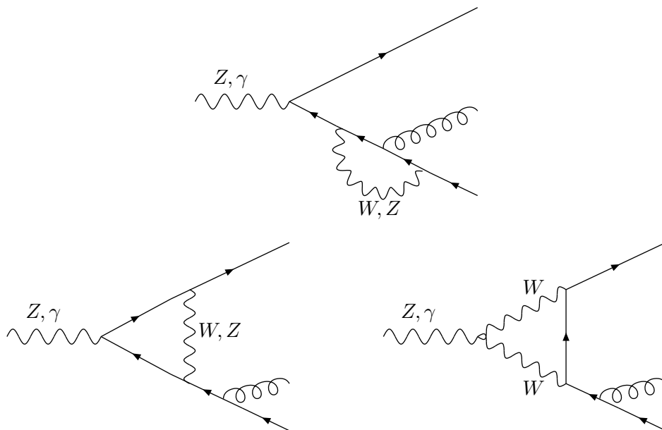
Figure 2: Vertex correction graphs. Again, same considerations as in the previous figure apply for the case of Goldstone bosons and there is a similar set of graphs in which the direction of the fermion line is reversed.
