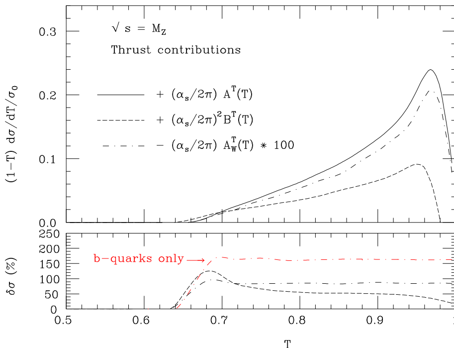
Figure 6: The LO, NLO-QCD and NLO-W contributions to the coefficient functions entering the integrated Thrust distribution, see eq. (4.10), for process (4.1) (top) and the relative size of the two NLO corrections (bottom), at \sqrt{s} = M_Z . The correction for the case of b -quarks only is also presented, relative to the LO results for process (4.2). (Notice that the \sim A_W terms have been plotted with opposite sign and multiplied by hundred for better presentation.)
