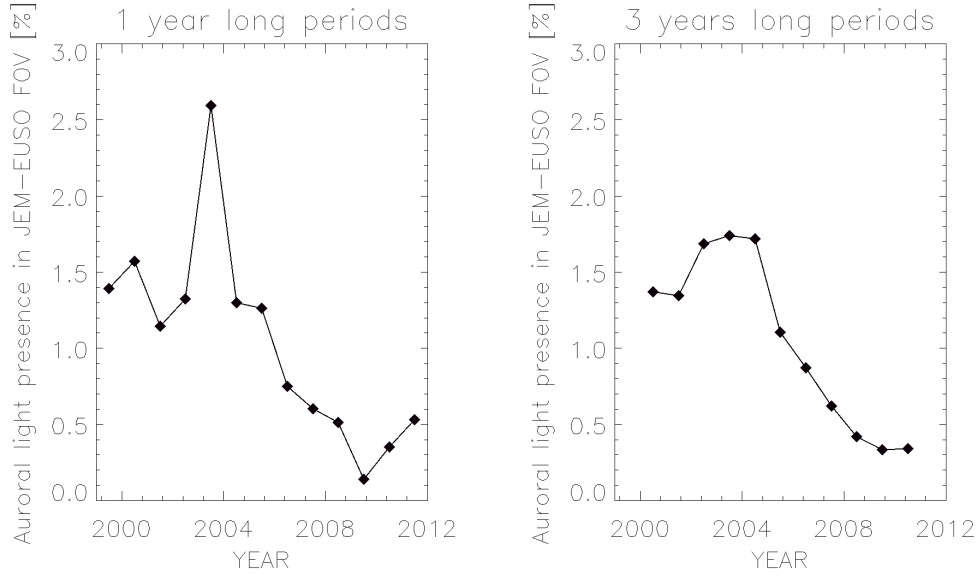
Figure 3: Left panel: Fraction of time f_{AL} in which auroral light restrains EAS measurements for one year long periods from 2000 to 2011. Right panel: Same as in the left panel, but integrating for 3-year periods.
