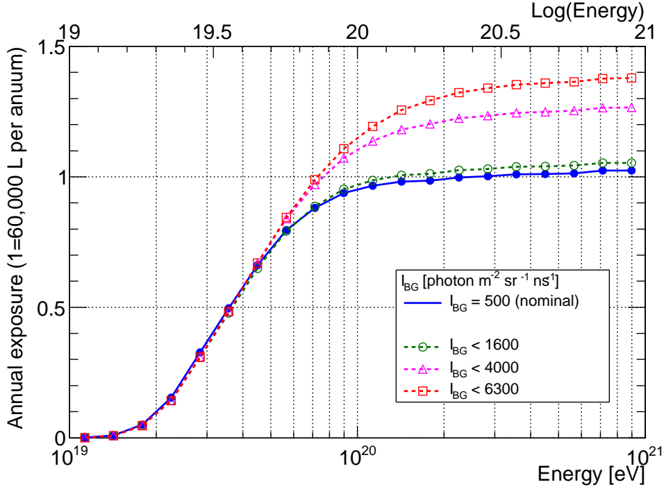
Figure 7: Exposure curve per year assuming the nominal background level of 500 photons \text{m}^{-2} \text{sr}^{-1} \text{ns}^{-1} (blue curve). The unit is defined 60,000 L per annum ( 1 \text{ L} = 1 \text{ km}^2 \text{sr yr} ). The other curves indicate, in arbitrary units, the relative exposure to the nominal one for different values of maximum acceptable background level.
