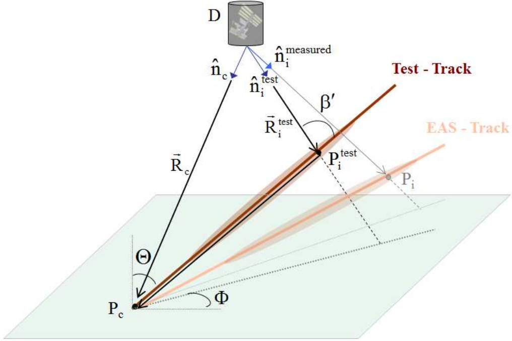
Figure 11: EAS observed with JEM-EUSO: Photons emitted by the shower reach the detector from certain directions \hat{n}_i, \hat{n}_j after traversing R_i, R_j in the atmosphere. The comparisons between the incident directions of the shower photons to those of a test EAS from different arrival directions allow to reconstruct \hat{\Omega}(\Theta, \Phi) .
