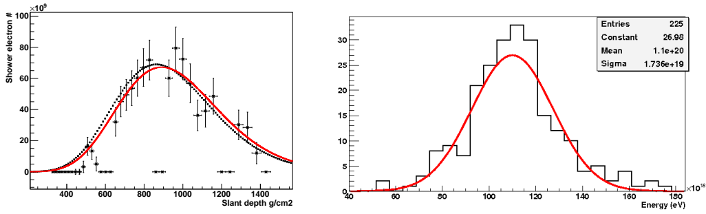
Figure 16: Left panel: Reconstructed shower profile of a typical simulated event. Data points indicate the reconstructed electron number as a function of depth after all in-instrument and atmospheric corrections have been applied. Black dashed curve shows the original profile, while the red line the reconstructed one from the fit of the data points. Right panel: Energy distribution of the events that are selected by the quality cuts. The results shown in the legend refer to the Gaussian fit of the distribution.
