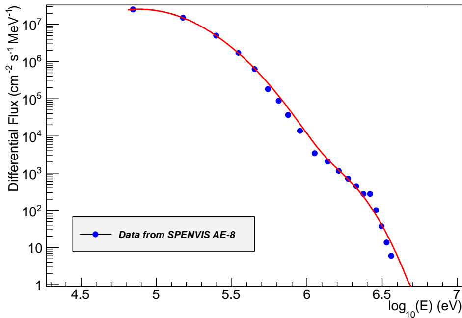
Figure 5: Differential flux of trapped electrons evaluated from SPENVIS AE-8 model for solar maximum period in the central region of the SAA. The continuous line represents the parametrization used for the simulation.
