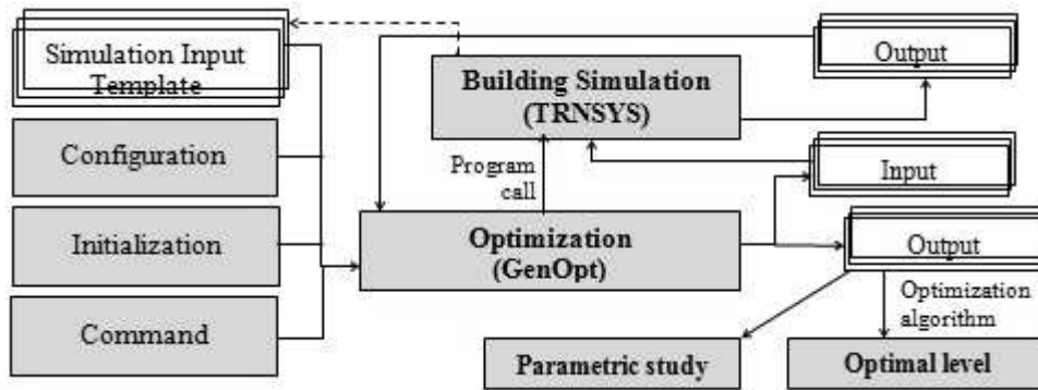
Figure 3. Simulation-optimization framework.
