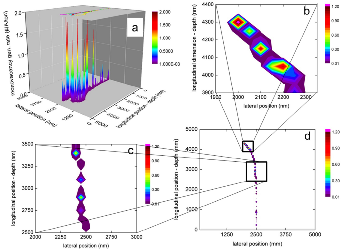
Fig. 1: Monte-Carlo simulation of the disordered region dense with monovacancies and interstitials following the single 8.3 MeV O ion implantation of silicon: a) the cumulative projection on a horizontal beam plane of all monovacancies, created by five different ion-projectiles and their recoil cascades, per unit length of a projectile (VGR); d) The surface contour plot of the VGR distribution generated by random chosen single ion cascade in material with entry point at (2500,0) nm; b) the enlarged area close to the end of an ion range, and c) the enlarged mid-range area corresponding to the disordered regions probed by differential DLTS measurement. VGR yields shown by colour bars are expressed in monovacancy per Angstrom units.
