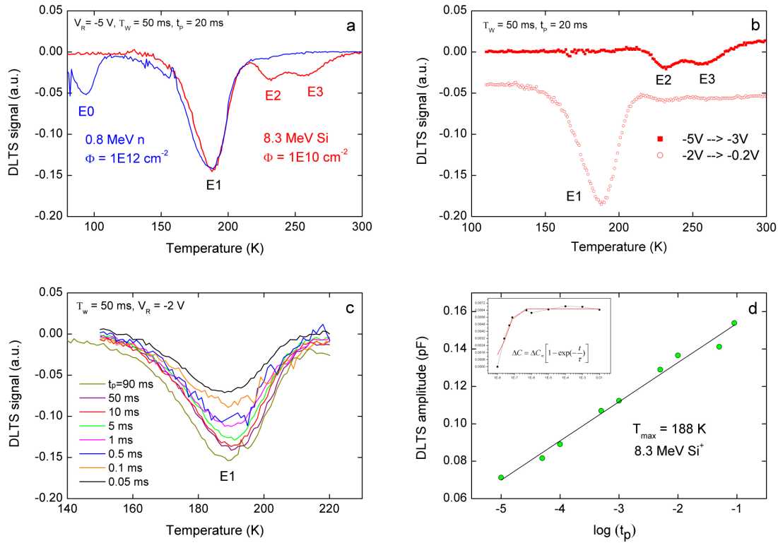
Fig.2. Results of DLTS spectroscopy performed on implanted silicon diodes: a) normalized DLTS spectra obtained by 8.3 MeV Si single ion implantation (red) and 0.8 MeV neutron irradiation (blue); b) depth profiling of the vacancy-rich surface side of the implant tail (circles) and interstitial-rich region near the implant peak (squares); c) section of DLTS spectra corresponding to E1 peak formed in the implant tail as function of a duration time of the filling pulse ( t_p ); d) results of carrier capture cross-section analysis of the E1 trap showing logarithmic behaviour typical for complex (cluster) defect structures. Inset in fig.2 (d) shows the exponential dependence of carrier capture cross section typical for point defects.
