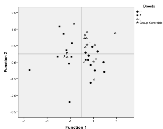
Figure 4 Plot of the two discriminant functions for classification of young bulls according to their breed.
