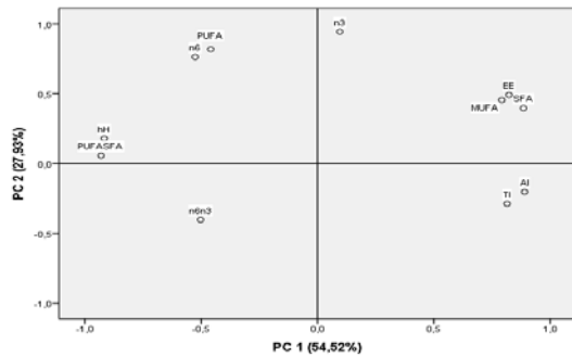
Figure 2 Plot of the first two PC loading vectors.
