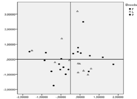
Figure 3 Plot of the first two PC score vectors.
