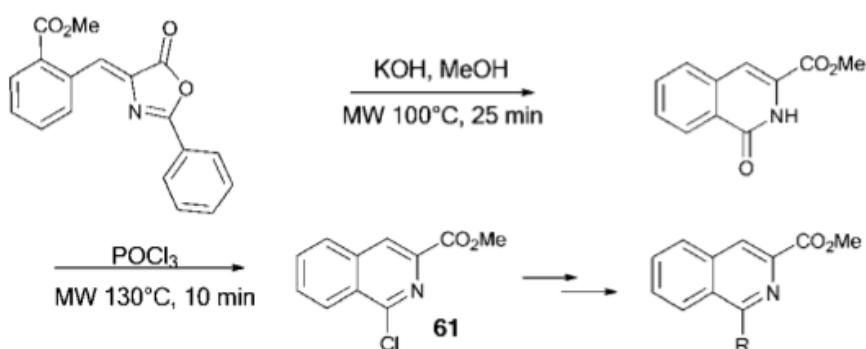
Scheme 42
