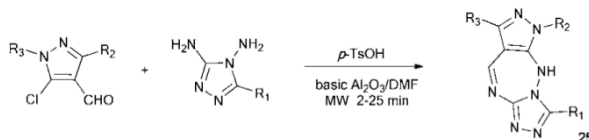
Scheme 19
