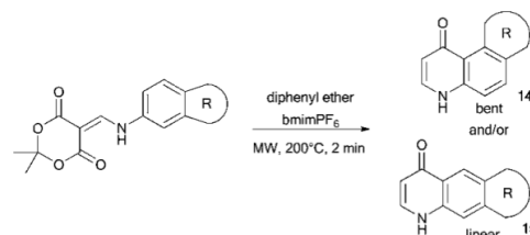
Scheme 12
