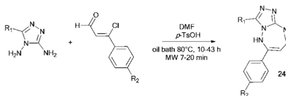
Scheme 18
