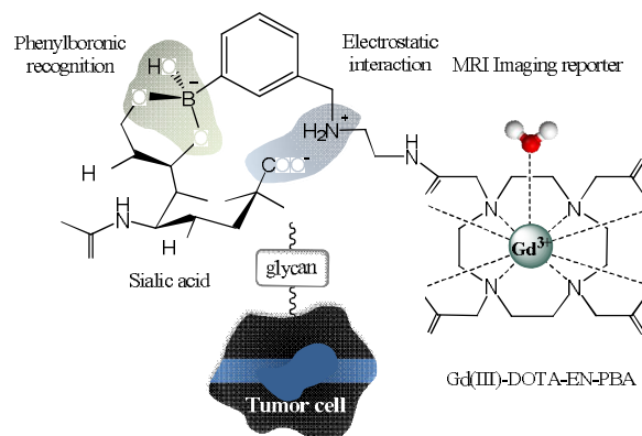
Figure 1. Schematic representation of sialic acid recognition by imaging reporter Gd(III)-DOTA-EN-PBA via diol-phenylboronic interaction on the surface of tumor cells.
