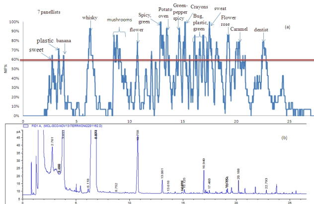
Figure 1. Aromagram showing the most important odoriferous regions for banana spirit (NIF \geq 60%) and chromatogram (b) with the corresponding retention times (min).
