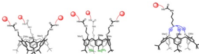
Figure 1: Calix[6]arene derivatives
