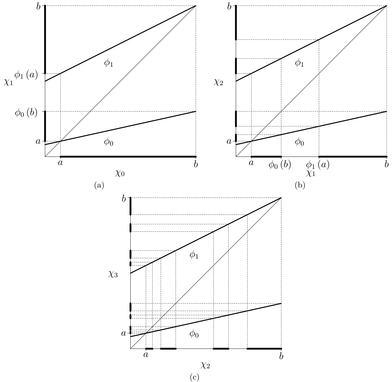
FIGURE 1: first three iterations of the IFS in (5) for \eta = s = 0.5 , A = 1 , \delta_\ell = 0.11 and \delta_u = 0.25 starting from the initial set [a, b] in t = 0 , with a = 1.282 and b = 2 .
