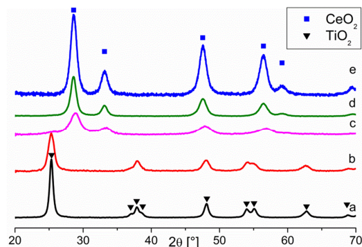
85 Fig. 1 . XRD of CeO 2 /TiO 2 mixed oxides: (a) TiO 2 (sol-gel); (b) 10% mol CeO 2 , CT10; (c) 50% mol CeO 2 , CT50; (d) 90% mol CeO 2 , CT90; (e) CeO 2
