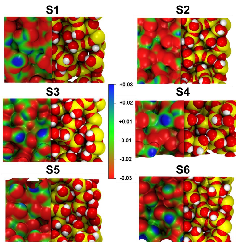
Figure 3. The six S1-6 inner faces of the MCM-41 pore walls. The right strip shows the space filled structure on top of which (left strip) the electrostatic potential is mapped on the electron density isosurface (isovalue: 0.0004 e ). Color scale shown in the picture.
