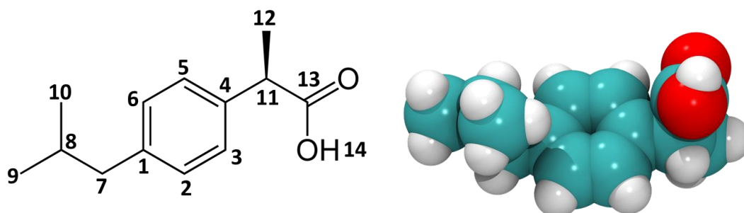
Figure 4. Structure of the 2-(4-isobutylphenyl)-propionic acid ( \text{H}_{18}\text{C}_{13}\text{O}_2 ), ibuprofen drug molecule. Left: 2D chemical structure with atom numbering. Right: 3D space filling model of the B3LYP-D* optimized most stable conformer.
