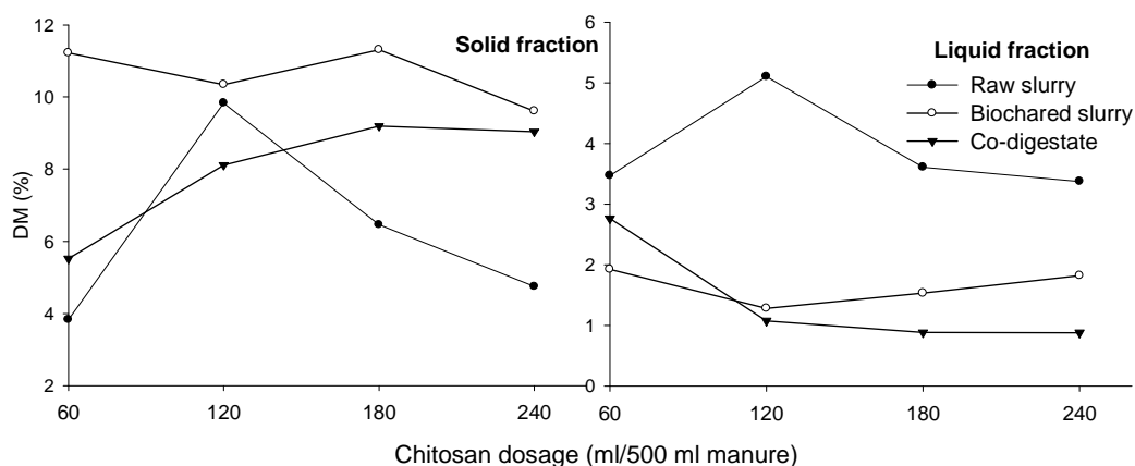
Figure 2. Solid and liquid fractions dry matter after different chitosan dosages addition to raw and biochared slurry and co-digestate prior to gravity drainage
