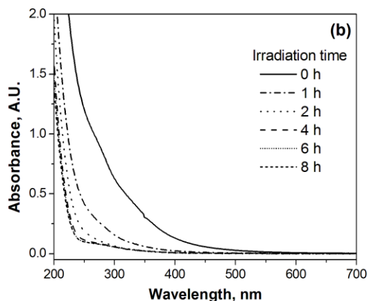
Figure 5. Time trends of the absorption spectra of \text{CVT230}_{\text{sol}} , as a function of the irradiation time, (a) without and (b) with \text{H}_2\text{O}_2 addition. \text{CVT230}_{\text{sol}} was separated before irradiation from a 500 \text{ mg L}^{-1} CVT230 solution.
