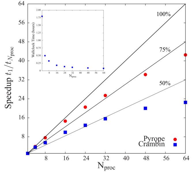
FIG. 3: (color online) Speedup of the calculation of the electrostatic potential on 3D grid of 250'000 points of pyrope (red circles) and crambin (blue squares) as a function of the number of processors used N_{\text{proc}} . The three black lines of decreasing thickness mark the 100%, 75% and 50% efficiency of the parallelism, respectively. The inset shows the reduction of the wall-clock time of the calculation in the case of crambin as a function of N_{\text{proc}} .
