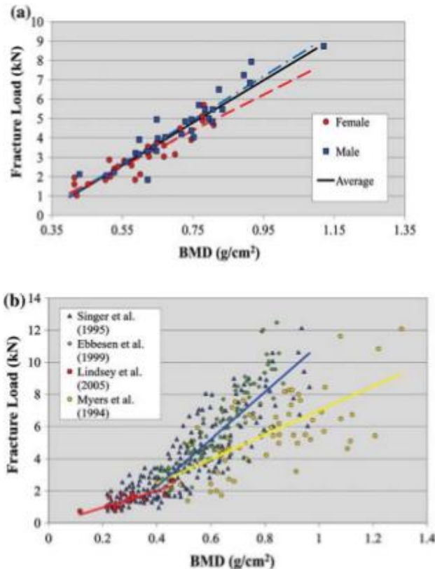
Fig. 5 Fracture load (FL) as a function of bone mass used in BFRM with underlying datasets (Nelson et al. 2009)
