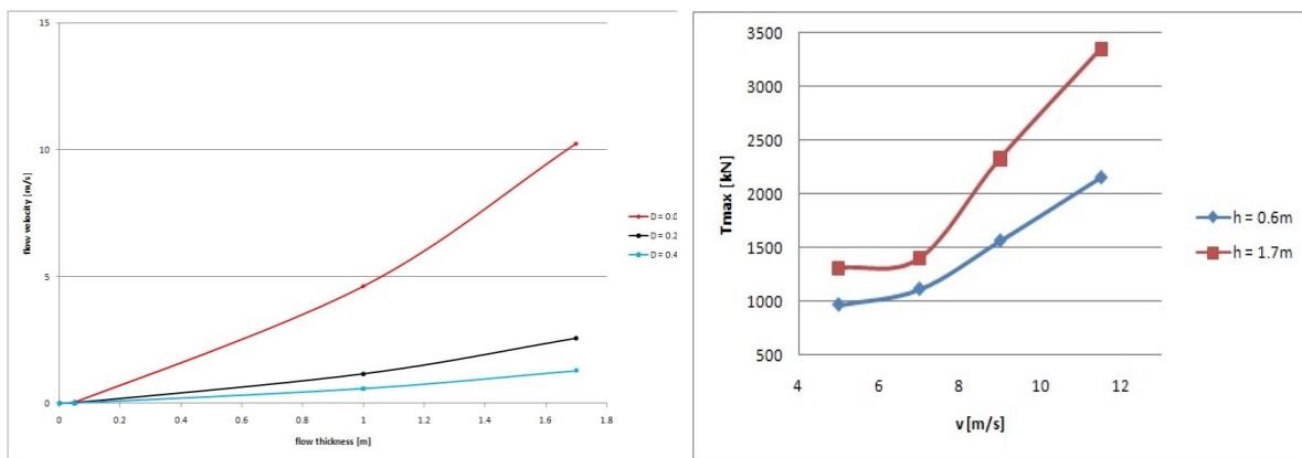
Fig. 7. (left) Variation of debris velocity with its thickness, according to different flow models (after Ferrero et al., 2015); the red lines specify the range of variation of the flow dept.(Right) Range of variation of maximum tensile force for cable 1 obtained using the simplified analytical model for different values of flow velocity and depositional height.
