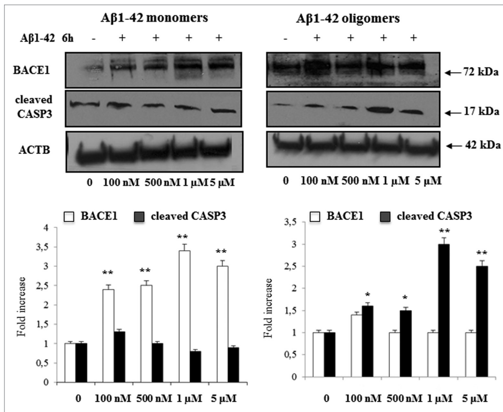
Figure 8. Treatment of differentiated SK-N-BE cells with different concentrations of Aβ1-42 monomers or oligomers does not modify the effects observed with the 1 μM concentration. BACE1 and CASP3 protein levels in differentiated SK-N-BE cells treated with a range (100 nM–5 μM) of Aβ1-42 monomers or oligomers for 6 h. We observed that monomers are not capable of increasing CASP3 levels even at higher concentrations, whereas they increase BACE1 protein levels at any concentration. Oligomers, in turn, fail to increase BACE1 levels at any concentration, but significantly increase cleaved CASP3 protein levels at all concentrations. The error bars represent standard deviations. Experiments were conducted in triplicate. *, significantly different from controls ( P < 0.05 ); **, significantly different from controls ( P < 0.02 ).
