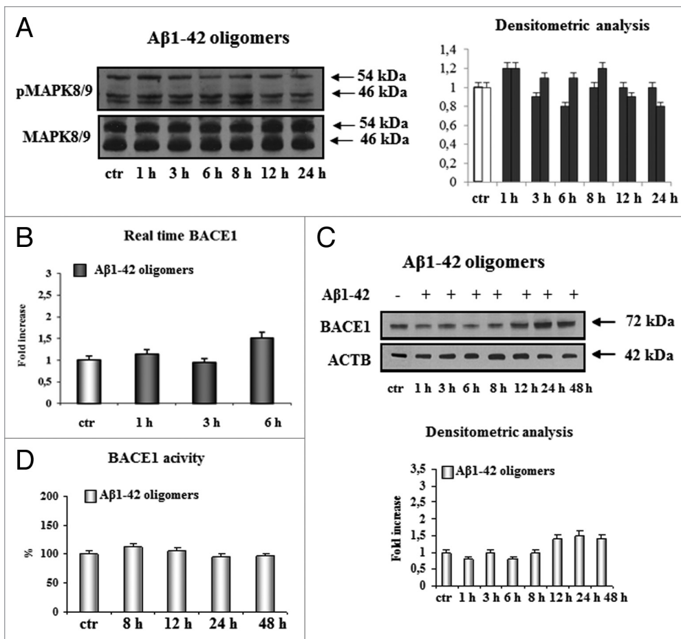
Figure 7. Treatment of differentiated SK-N-BE cells with 1 \mu M A \beta 1-42 oligomers does not affect BACE1 expression and the JNK pathway. (A) Nuclear pJNK protein levels in differentiated SK-N-BE treated with A \beta 1-42 oligomers up to 24 h. A \beta 1-42 oligomers do not activate JNK phosphorylation in nuclear fraction of differentiated SK-N-BE cells. (B–D) BACE1 expression, protein levels, and activity in cells treated with A \beta 1-42 oligomeric preparation. Treatment of cells with A \beta 1-42 oligomers was not followed by significant induction of BACE1 mRNA, protein levels, and activity. The error bars represent standard deviations. Experiments were conducted in triplicate.
