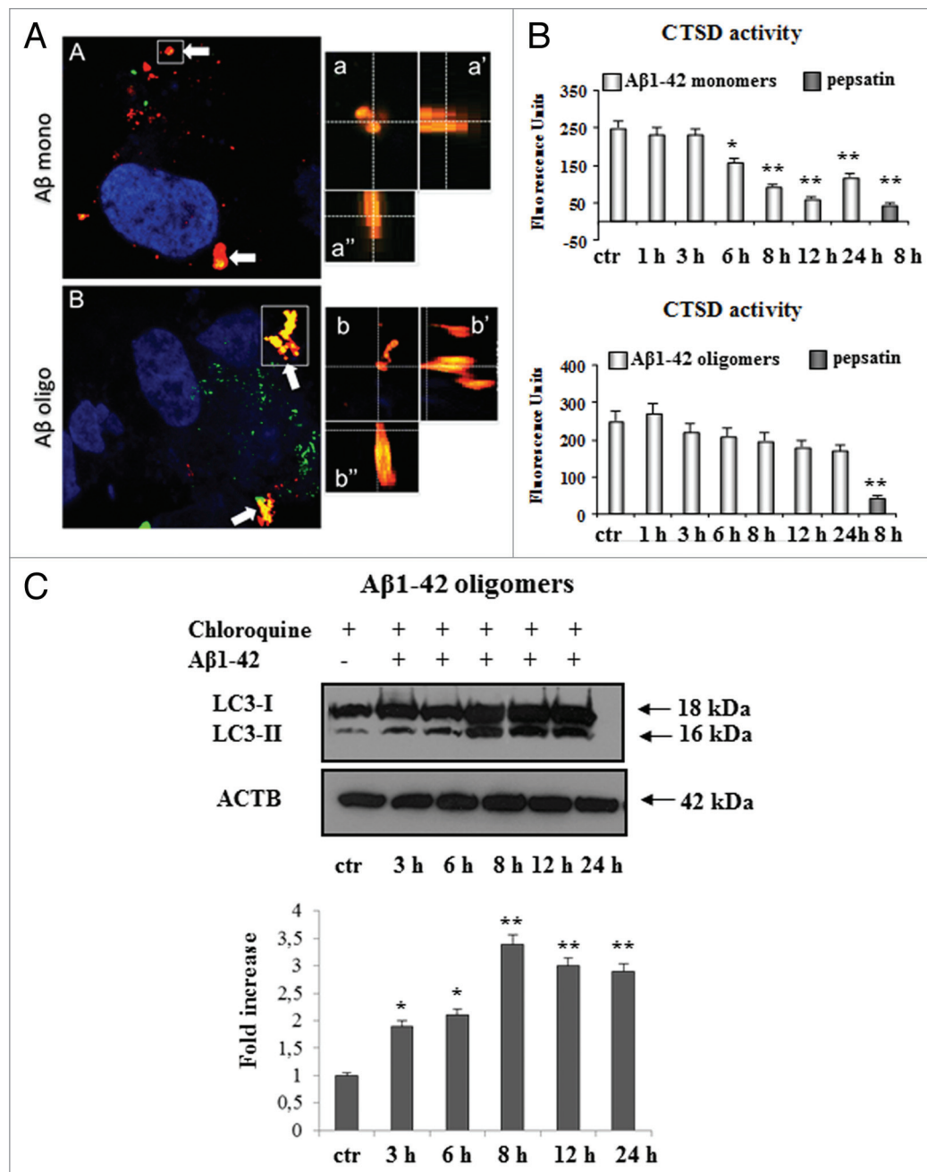
Figure 3. Treatment of differentiated SK-N-BE cells with 1 \mu M A \beta 1-42 monomers affects autophagic flux through impairment of lysosomal activity. (A) Lysosomal-associated membrane protein 1 (LAMP1) immunostaining after 24 h treatment with the A \beta species. Cells treated with 1 \mu M A \beta 42 monomers and oligomers for 24 h were stained, after fixation and permeabilization, with LAMP1 monoclonal and A \beta 42 polyclonal antibodies. After washing in PBS, sections were incubated with secondary antibodies raised in different species: 1:200 cyanine 3-conjugated donkey anti-mouse secondary antibody and 1:100 cyanine 2-conjugated anti-rabbit secondary antibody) with 1% BSA in PBS. For counterstaining, cells were incubated for 3 min with DAPI diluted 1:50 in methanol 0.1 M and rinsed with PBS. As shown, lysosomal vesicles are formed and also there is a colocalization with lysosomes and the 2 A \beta 1-42 preparations. (B) CTSD activity evaluation in SK-N-BE differentiated cells after treatments with the 2 A \beta 1-42 preparations. Only treatment with A \beta 1-42 monomers was followed by a significant decrease in the CTSD activity after 6 h and up to 24 h. Pepsatin, used as a positive control induced ~80% inhibition of the enzyme activity after 8 h of incubation. (C) LC3-II protein levels in SK-N-BE cells pretreated with 100 \mu M chloroquine for 24 h and then treated with A \beta 1-42 oligomeric preparation for 8 h. Pretreatment of cells with the lysosomal inhibitor was able of mediating a strong and significant increase in LC3-II protein levels, with a trend almost similar to monomers. The error bars represent standard deviations. Experiments were conducted in triplicate. *, significantly different from controls ( P < 0.05 ); **, significantly different from controls ( P < 0.02 ).
