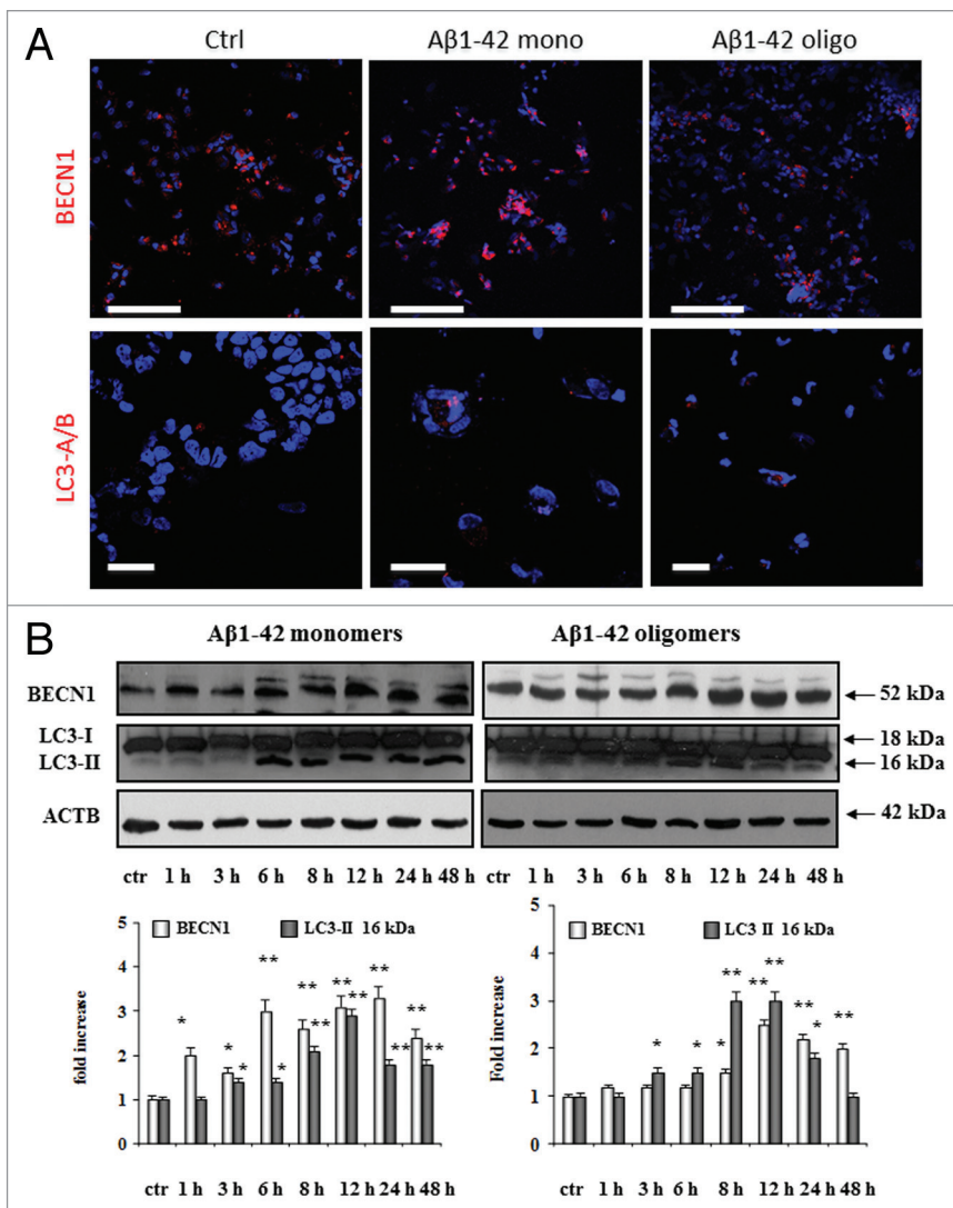
Figure 1. Treatment of differentiated SK-N-BE cells with 1 \mu M A \beta 1-42 monomers and oligomers significantly increase BECN1 and LC3-I and LC3-II fluorescence intensity and protein levels. (A) Cells treated with 1 \mu M A \beta 42 monomers and oligomers for 24 h were stained, after fixation and permeabilization, with BECN1 or LC3 antibodies. After washing in PBS, sections were incubated with secondary antibodies raised in different species: 1:200 cyanine 3-conjugated donkey anti-mouse secondary antibody and 1:100 cyanine 2-conjugated anti-rabbit secondary antibody with 1% BSA in PBS. For counterstaining, cells were incubated for 3 min with DAPI diluted 1:50 in methanol 0.1 M and rinsed with PBS. After 24 h both monomeric and oligomeric A \beta 1-42 preparations increased BECN1 immunoreactivity; however a higher number of positive cells were observed after treatment with the monomeric preparation. (B) BECN1 and LC3-I/II protein levels in cells treated with 1 \mu M A \beta 42 monomers and oligomers at different time points up to 48 h. Both preparations were able to significantly increase BECN1 levels, but the increase was more pronounced with monomers than with oligomers (up to 3-fold with monomers vs. 2.5-fold with oligomers). Examination of LC3-II levels also showed an increase in protein levels for both monomeric and oligomeric preparations. Monomers of A \beta 1-42 led to a marked and significant increase in LC3-II protein levels that started at 3 h and was still present after 48 h of treatment, whereas oligomers produced a transient increase that was no longer present after 8 h to 12 h of incubation. The error bars represent standard deviations. Experiments were conducted in triplicate. *, significantly different from controls ( P < 0.05 ); **, significantly different from controls ( P < 0.02 ).
