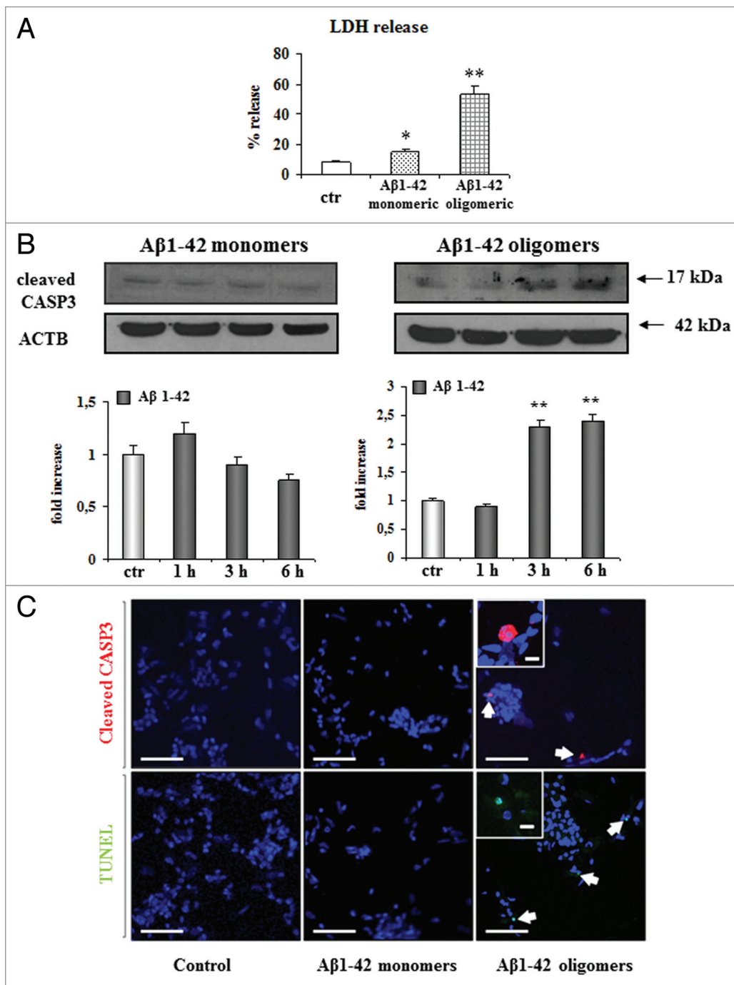
Figure 4. Treatment of differentiated SK-N-BE cells with 1 \mu M A \beta 1-42 oligomers, but not monomers, significantly increases LDH release in the medium as well as cleavage of CASP3 and DNA fragmentation. (A) LDH release in differentiated SK-N-BE treated with A \beta 1-42 oligomers as well as monomers for 24 h. The treatment of differentiated neuroblastoma cells with oligomeric A \beta 1-42 preparation induced a more severe (~60% vs. 20%) release of LDH compared with the monomeric form. (B) Cleaved-CASP3 protein levels in cells treated with different A \beta species. We found that only oligomeric A \beta 1-42, significantly increased (2.5-fold) the cleavage of CASP3 at 3 h and 6 h of incubation. (C) Cells treated with both oligomers and monomers of A \beta 1-42 for 6 h were fixed, permeabilized, and stained with polyclonal antibodies against cleaved CASP3 (red) or with the DNA fragmentation stain TUNEL (green), and then analyzed by confocal microscopy. Monomers did not change cell number compared with controls, whereas oligomers strongly decreased it (oligomers: 61% increase in apoptotic nuclei vs. control; monomers: 18% increase in apoptotic nuclei vs. controls). Arrows indicate puncta of either cleaved CASP3 or TUNEL staining. Higher magnification views of given areas are encapsulated in squares. The nuclear stain DAPI (4,6 diamidino-2-phenylindole, blue) was used to stain cells. Scale bars: 100 \mu m, or 15 \mu m for higher magnification views. The error bars represent standard deviations. Experiments were conducted in triplicate. *, significantly different from controls ( P < 0.05 ); **, significantly different from controls ( P < 0.02 ).
