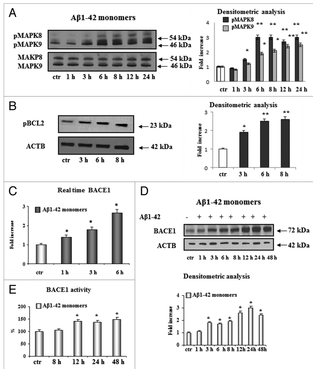
Figure 6. Treatment of differentiated SK-N-BE cells with 1 \mu M A \beta 1-42 monomers increases BACE1 expression and activity through the activation of the MAPK/JNK pathway. (A) Nuclear pMAPK/JNK protein levels in differentiated SK-N-BE treated with A \beta 1-42 monomers up to 24 h. The treatment was followed by a robust activation of the MAPK/JNK pathway, as shown by the significant increase (~3 to 2.5-fold) in levels of phospho-MAPK/JNK in nuclear fractions. (B) Phosphorylated BCL2 protein levels of in cytosolic fractions of cells treated with monomers up to 8 h. As expected with the activation of the MAPK/JNK pathway, cells treated with A \beta 1-42 monomers revealed a significant increase (~2.5-fold) in BCL2 phosphorylation (C-E) BACE1 expression, protein levels, and activity in cells treated with A \beta 1-42 monomeric preparation. Treatment of cells with A \beta 1-42 monomers induced a 1.5- to 2.5-fold increase in BACE1 mRNA, as well as a 100% to 200% increase in BACE1 protein levels and a 35% increase in BACE1 activity. The error bars represent standard deviations. Experiments were conducted in triplicate. *, significantly different from controls ( P < 0.05 ); **, significantly different from controls ( P < 0.02 ).
