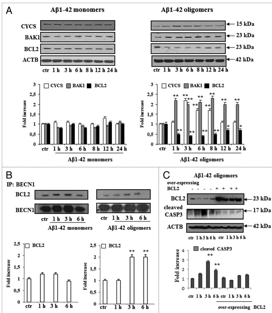
Figure 5. Treatment of differentiated SK-N-BE cells with 1 \mu M A \beta 1-42 oligomers significantly increases CYCS and BAK1 and decreases BCL2 levels and allows the interaction between BCL2 with BECN1. (A) CYCS, BAK1 and BCL2 protein levels in differentiated SK-N-BE cells treated with A \beta 1-42 oligomers as well as monomers up to 24 h. Treatment with oligomeric A \beta 1-42 increased the CYCS release (100 - 120%) after 3 h and up to 24 h, and BAK1 protein levels (120–150%) after 1 h and up to 24 h, whereas BCL2 levels resulted significantly decreased (50%). Treatment of cells with monomeric preparations of A \beta 1-42 did not affect these parameters. (B) Cells treated with A \beta preparations were immunoprecipitated with polyclonal BECN1 antibody and revealed with monoclonal BCL2 antibody. We found that BCL2 is linked to BECN1 only after 3 h to 6 h of treatment with A \beta 1-42 oligomers. (C) BCL2 and cleaved CASP3 protein levels in differentiated SK-N-BE control and overexpressing BCL2 cells treated with 1 \mu M A \beta 1-42 oligomers. BCL2 overexpression was able to attenuate the cleavage of CASP3 mediated by oligomers. The error bars represent standard deviations. Experiments were conducted in triplicate. **, significantly different from controls ( P < 0.02 ).
