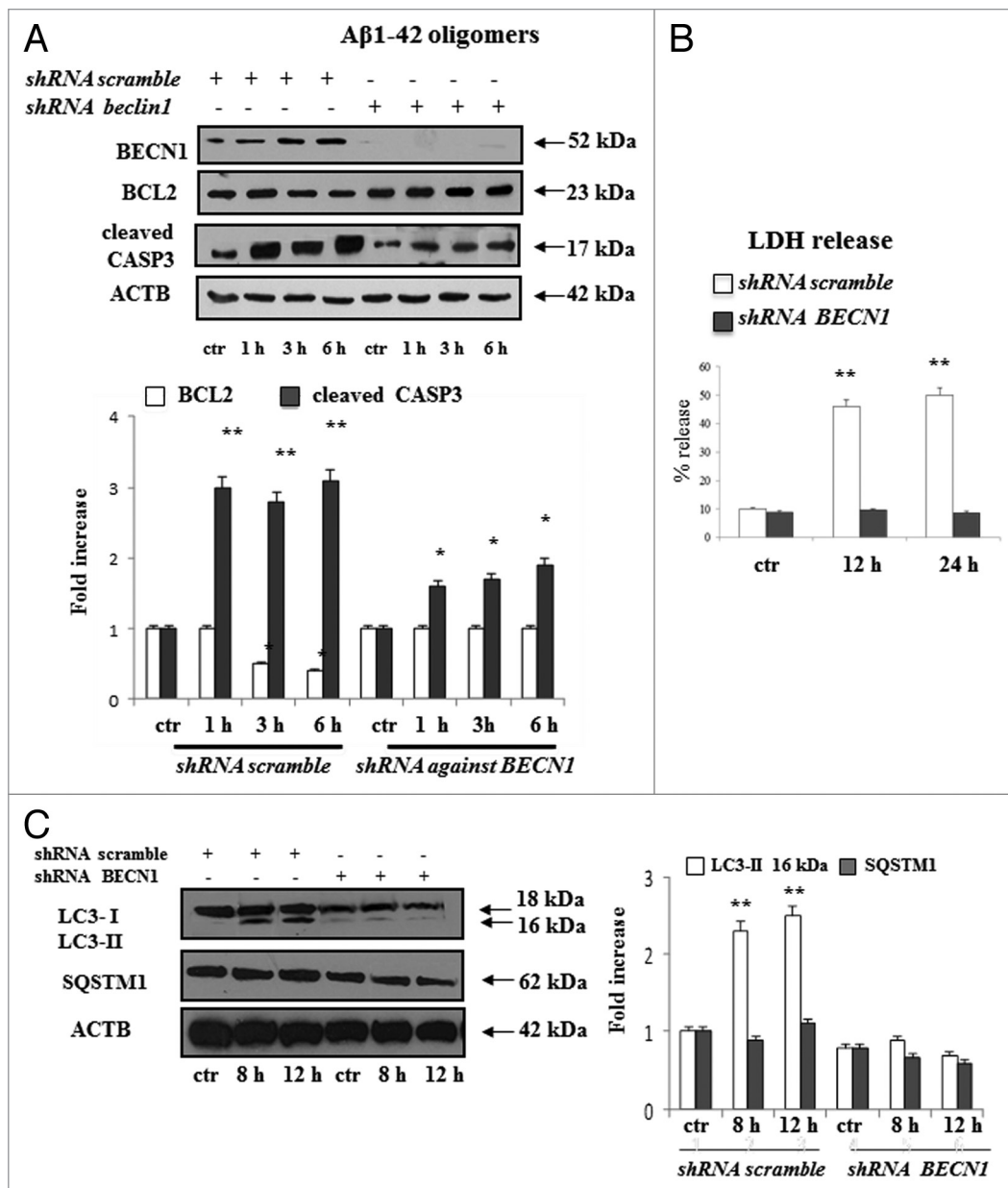
Figure 9. BECN1 is needed for the toxicity mediated by A \beta 1-42 oligomers. (A) BECN1, BCL2, and cleaved CASP3 protein levels in SK-N-BE cell lines stably expressing a specific shRNA against BECN1 or scrambled shRNA treated with A \beta 1-42 oligomers up to 6 h. BECN1 is observed only in cells expressing scrambled shRNA while a band corresponding to the protein is not observed in cell expressing shRNA against BECN1 . BCL2 protein levels remain unchanged in cells silenced for BECN1 treated with A \beta 1-42 oligomers up to 6 h, whereas cleaved CASP3 are protected but slightly significant with respect to untreated cells. (B) LDH release in culture medium in control as well as in silenced neuroblastoma cells treated with A \beta 1-42 oligomers for 24 h. In silenced cells oligomers failed to induce necrotic cell death after 12 h and 24 h of treatment. (C) LC3-II and SQSTM1 protein levels in cells with and without silencing for BECN1 and treated with oligomers of A \beta 1-42 for 8 h and 12 h. The absence of BECN1 lowered the basal levels of both LC3 and SQSTM1 and treatment of cells with the oligomeric preparation of A \beta 1-42 did not modify this trend. The error bars represent standard deviations. Experiments were conducted in triplicate. *, significantly different from controls ( P < 0.05 ); **, significantly different from controls ( P < 0.02 ).
