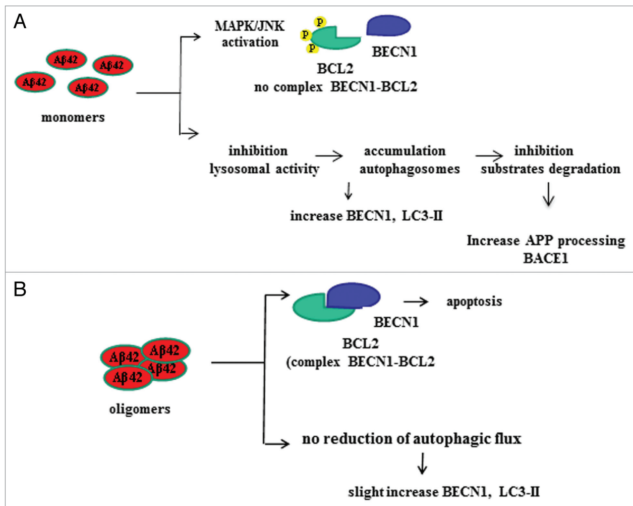
Figure 11. Proposed effects on autophagy and apoptosis elicited by A \beta 1-42 monomers and oligomers. (A) Monomers impede formation of the BCL2-BECN1 complex by activation of the MAPK/JNK pathway that phosphorylates BCL2. Monomers also cause early endosome accumulation due to an inhibitory action on lysosomal activity, resulting in intracellular accumulation of autophagosomes with elevation of levels of BECN1 and LC3-II, and inhibition of substrate degradation. (B) Oligomers favor the formation of the BCL2-BECN1 complex leading to apoptosis. They also cause a less profound increase in BECN1 and LC3-II levels and do not affect the autophagic flux.
