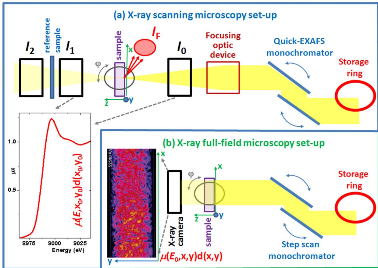
Figure 9. Schematic views of the basic set-up for spatially resolved X-ray absorption spectroscopy. Part (a): scanning monochromatic \mu\text{-beam} set-up. This set-up contains all the elements (i)-(v) of a conventional XAFS beam line (detection in transmission mode via I_0 and I_1 , in fluorescence mode via I_0 and I_F and edge calibration via I_2 , see Figure 4a). In addition it is equipped with focusing optics (Fresnel zone plates, 313 or compound refractive lens, 314-316 or Kirkpatrick–Baez mirrors, 317 or tapered capillaries 318 ), a quick-EXAFS monochromator and a sample stage with rotation ( \varphi ) and high precision ( x,y ) translations. Part (b): full-field imaging set-up. It is equipped with a standard step-scan monochromator, a high- (x,y) resolution X-ray camera, a sample stage with rotation ( \varphi ) and medium precision ( x,y ) translations. Both set-ups allow tomographic data acquisitions. The insets of parts (a) and (b) reports the outputs of the single step of each acquisition: a full XAFS spectrum of a single (x_0, y_0) point and a full transmission map recorded at a single energy E_0 . For scanning polychromatic \mu\text{-beam} , see the set-up reported in Figure 4b. Unpublished figure, inspired from the sketches reported in Refs. 71,336,337 The inset of part (b) has been reproduced with permission from Ref. 338 Copyright 2006 American Chemical Society.
