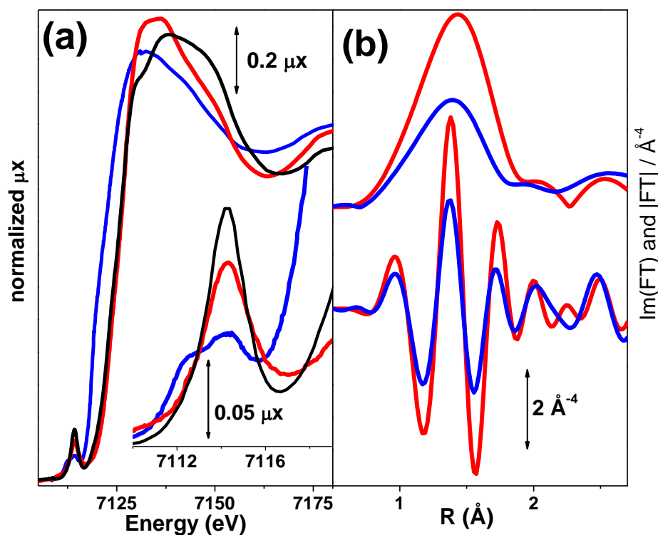
Figure 26. Part (a): XANES spectra of Fe-silicalite activated at 1073 K (blue line), and subsequent oxidation with N_2O at 523 K (red line). For comparison also the spectrum of the sample with template (i.e. of Fe^{3+} in T_d symmetry) is reported as black curve. The inset shows the magnification of the pre-edge peaks. Part (b): k^3 -weighted, phase uncorrected, FT of the EXAFS spectra of Fe-silicalite activated at 1073 K (blue curve), and after subsequent oxidation with N_2O at 523 K (red curve). Top and bottom curves refer to the moduli and the imaginary parts, respectively. Adapted with permission from Ref. 787 Copyright 2005 American Chemical Society.
