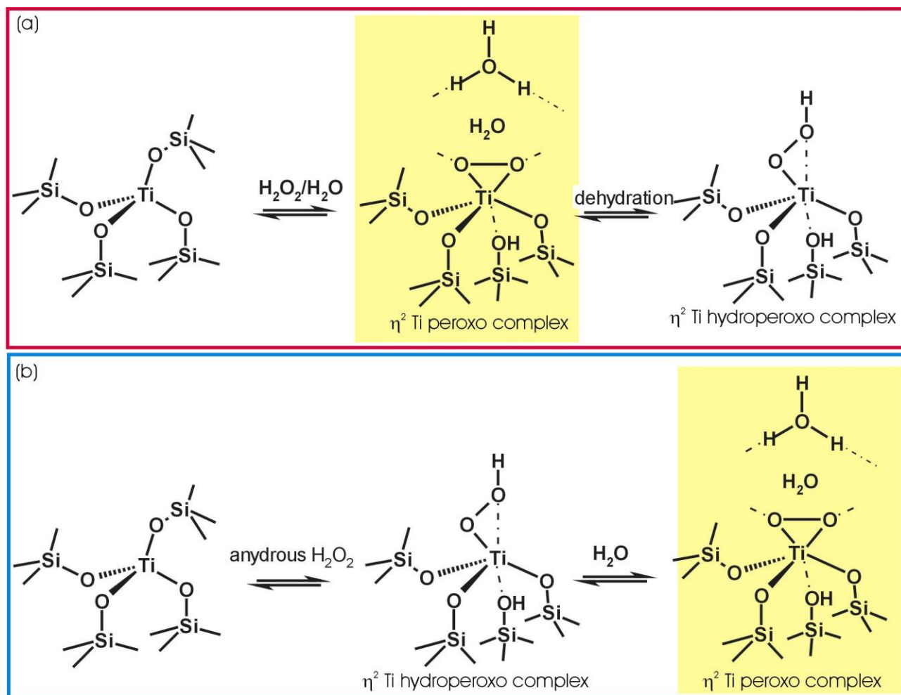
Scheme 6. Part (a): Representation of equilibria between TiO 4 framework species and side-on \eta^2 Ti peroxo complexes inside TS-1 channels upon dosage of H 2 O 2 /H 2 O (left) and between side-on \eta^2 Ti peroxo and end-on \eta^2 Ti hydroperoxo complexes upon dehydration (right). Part (b): Representation of equilibria between TiO 4 framework species and \eta^2 end-on Ti hydroperoxo complexes upon dosage of anhydrous H 2 O 2 (left) and between end-on \eta^2 Ti hydroperoxo and \eta^2 side-on Ti peroxo complexes upon hydration (right). Reproduced with permission from Ref. 886 Copyright 2007 Royal Society of Chemistry.
