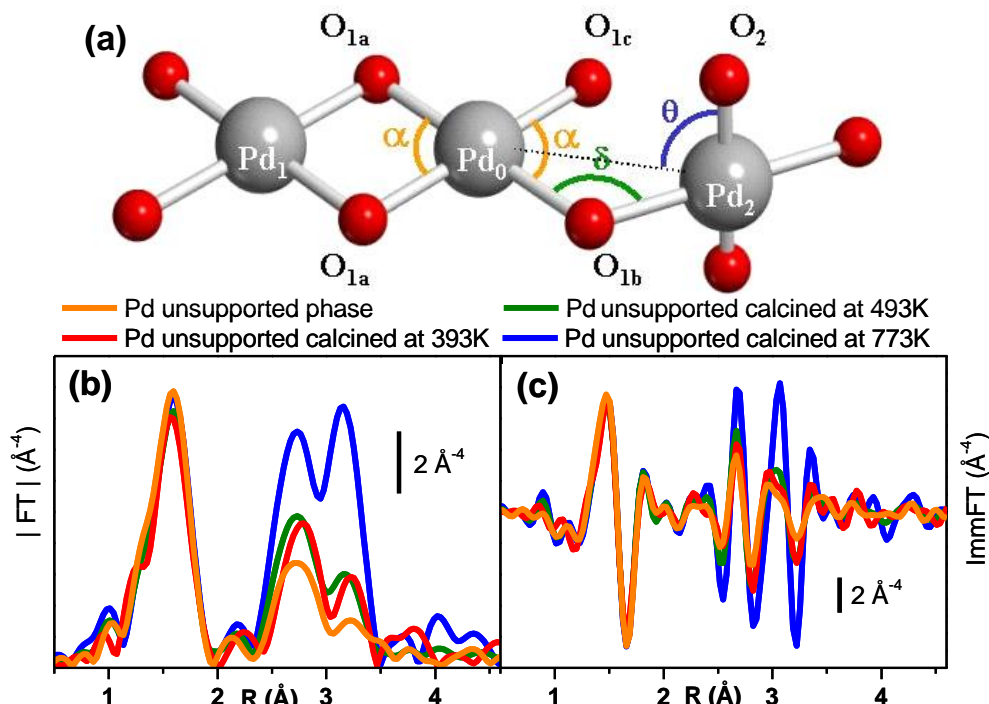
Figure 51 . Part (a) \text{Pd}(\text{OH})_2 cluster used to model the EXAFS signal up to 4.1 \text{ \AA} around the absorbing Pd atom (labeled as \text{Pd}_0 ). Gray and red spheres represent Pd and O atoms, respectively. H atoms, unable to contribute significantly to the EXAFS signal, have been omitted. The model has been constructed from the studies of Troitskii, et al. 1586 The structural parameters optimized in the EXAFS fit are the Pd-O first shell distance (considered equivalent for \text{O}_{1a} , \text{O}_{1b} and \text{O}_{1c} atoms), the \text{Pd}_0\text{-Pd}_1 , \text{Pd}_0\text{-Pd}_2 and \text{Pd}_0\text{-O}_2 distances and the corresponding Debye-Waller factors. The angles \alpha and \delta differs from the ideal 90^\circ of the square planar geometry in order to account for the optimized \text{Pd}_0\text{-Pd}_1 , \text{Pd}_0\text{-Pd}_2 and \text{Pd-O}_1 distances. As the two \text{PdO}_4 units centered in \text{Pd}_0 and \text{Pd}_2 are linked via an unique oxygen bridge ( \text{O}_{1b} ) the \text{PdO}_4 unit centered in \text{Pd}_2 is, in principle, free to rotate. The optimized \text{Pd}_0\text{-O}_2 distance allows to evaluate the
