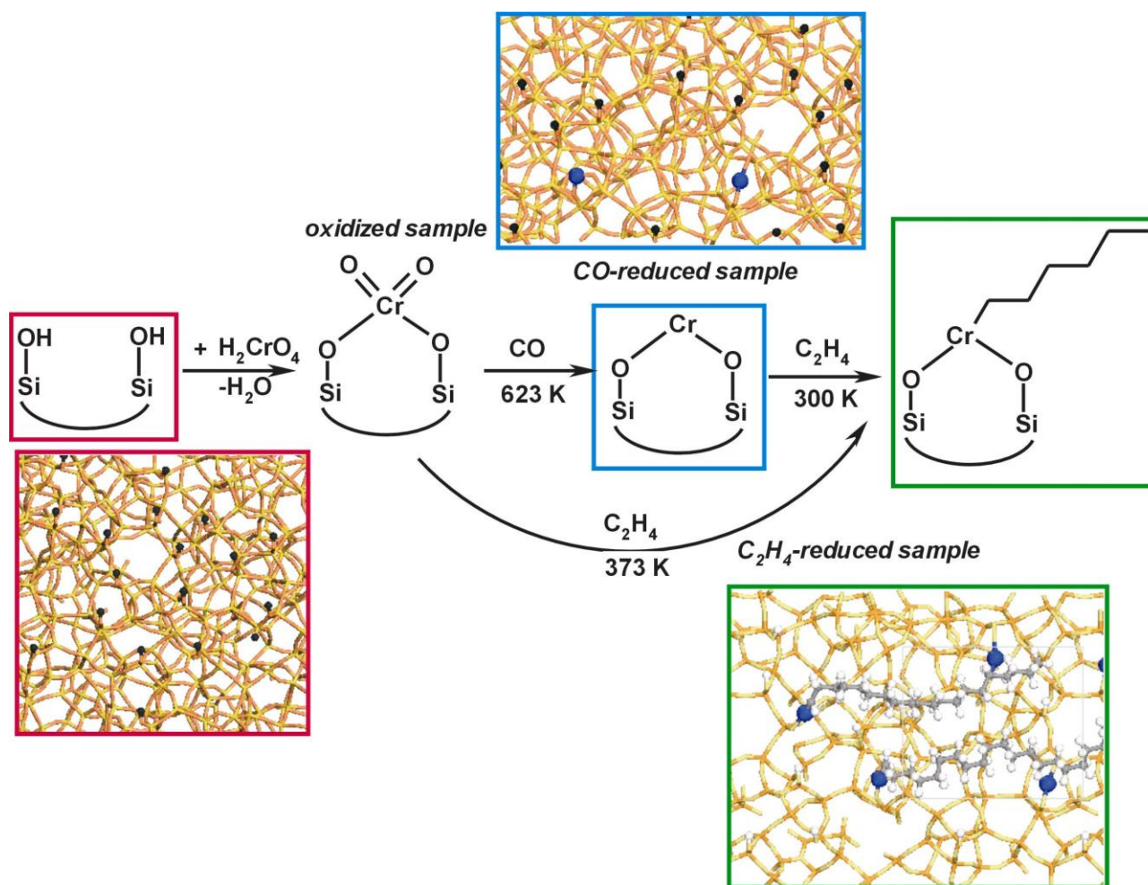
Figure 42. Schematic representation of the synthesis procedure for the \text{Cr}/\text{SiO}_2 Phillips catalyst (see text for a detailed description). In the insets, red and yellow sticks connect together silicon and oxygen atoms respectively; the big blue balls represent \text{Cr}(\text{II}) ions, while the little gray and white (black) balls represent carbon and hydrogen atoms, respectively. Unpublished Figure.
