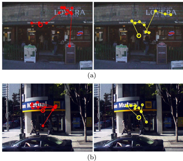
Fig. 11 Scan paths generated under the look for text for pictures from Microsoft dataset when other semantic objects (faces, people) are embedded in the picture together with text. Left (in red colour), scan path obtained eye-tracking a human observer; right, model output
