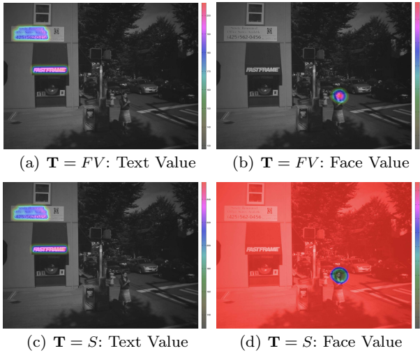
Fig. 5 The initial value probability maps P(\mathbf{V}_\ell(0)|\mathbf{R}(0), \mathbf{T}) calculated by weighting, at each spatial location, the estimated object maps (text and face) through the numerical payoff chosen for the given task \mathbf{T} (see text for details). The input image is the one used for the example in Fig. 4. Free view (FV): P(\mathbf{V}_{text}(0)|\mathbf{R}(0), FV) 5(a) and P(\mathbf{V}_{face}(0)|\mathbf{R}(0), FV) 5(b). Search for text (S): P(\mathbf{V}_{text}(0)|\mathbf{R}(0), S) 5(c) and P(\mathbf{V}_{face}(0)|\mathbf{R}(0), S) 5(d). Probabilities, superimposed on the foveated image, have been scaled between [0, 255] and colour coded, red colour denoting high probability, grey colour low probability.
