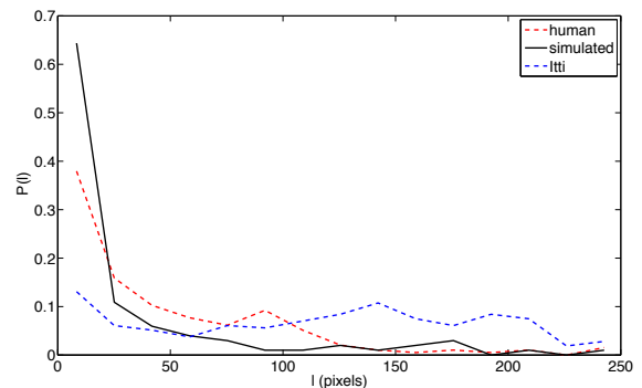
(a) Gaze shift amplitude distribution
