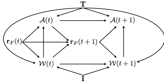
Fig. 2 The model represented as a dynamic Probabilistic Graphical Model. \mathcal{A}(t) stands for the ensemble of time-varying random variables (RVs) defining the oculomotor action setting (for short, the action component); \mathcal{W}(t) is the ensemble of time-varying RVs characterising the scene as actively perceived by the observer (the perception component). The gaze shift \mathbf{r}_F(t) \rightarrow \mathbf{r}_F(t+1) ties the dynamics of both components, and the scan path \{\mathbf{r}_F(1), \mathbf{r}_F(2), \dots\} is the result of an action-perception loop performed by the observer on an input image \mathbf{I} under a given task \mathbf{T} . Here, the evolving loop is unrolled for two time slices, respectively, t and t+1 .
