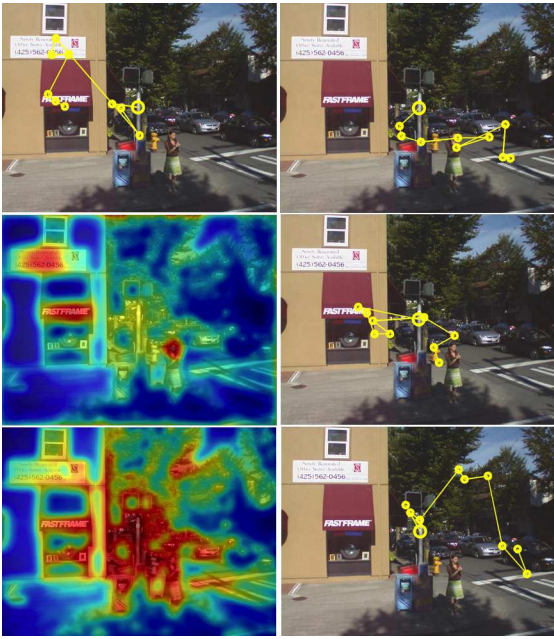
Fig. 6 Inhibition of levels of representation and control. Top row: scan path generated when the given task T is “Look for text”, similarly to Fig. 4 (left); scan path generated when the model simulates a “Look for people” task (right). Middle row, no task and value assigned, but object likelihood is still computed: the foveated priority map L (left, red colour coding for high priority locations, blue for low priority) and one generated scan path (right). Bottom row: when the object likelihood is not computed, the priority map collapses to a classic early saliency but modulated by foveation (left); a corresponding scan path (right). All maps are depicted at the same resolution (HR) of the original image I for visualization purposes
