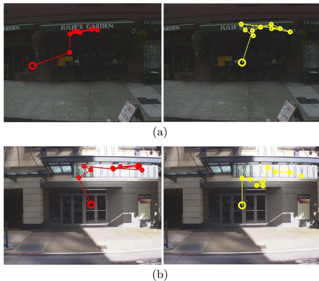
Fig. 10 Scan paths generated under the “Look for text regions” task for pictures from the Microsoft dataset, where text is the main semantic object class. Left (in red colour), scan path obtained eye-tracking a human observer; right, model output
