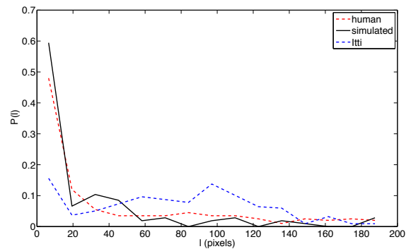
(a) Gaze shift amplitude distribution
