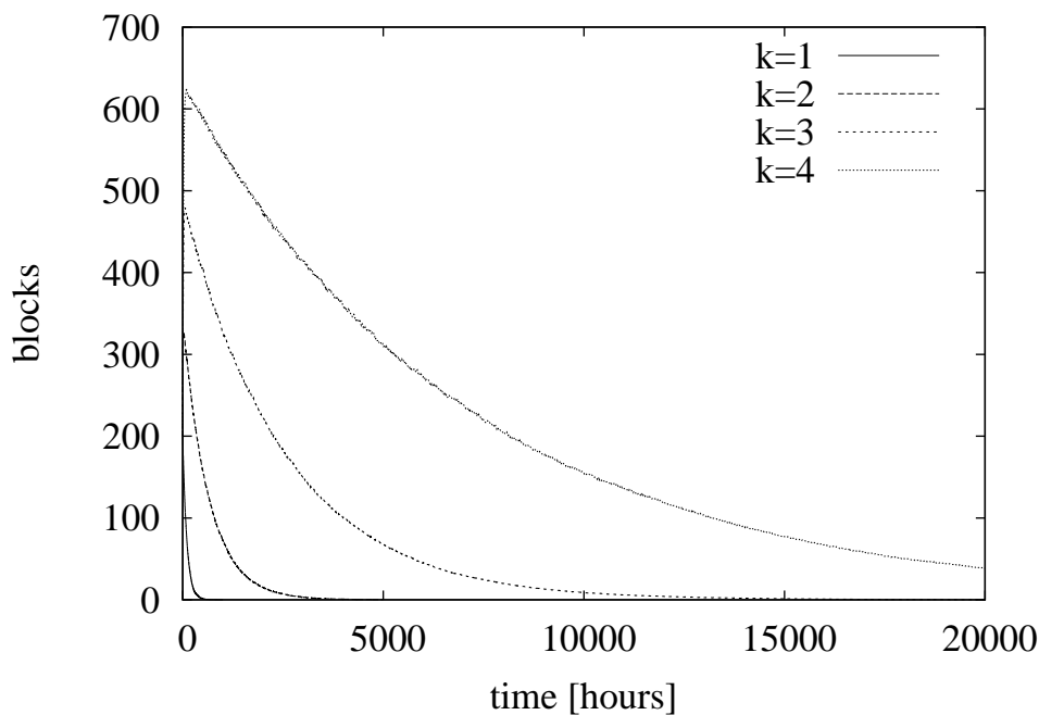
Figure 17: Blocks and chunks availability as function of time: average number of blocks (large time scale).
