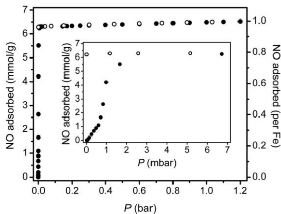
Figure 1. Adsorption of NO in \text{Fe}_2(\text{dobdc}) at 298 K; closed and open symbols represent adsorption and desorption, respectively. Saturation is nearly achieved by 7 mbar (inset).
