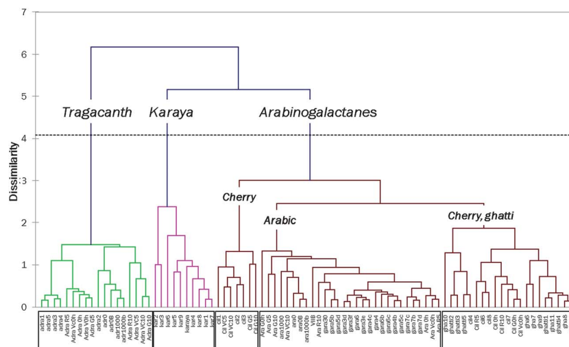
Fig. 3 Dendrogram obtained from a set of 85 samples of various kinds of gums.
