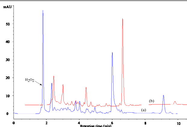
Fig. 6. Chromatograms obtained after 10 min of MET irradiation in the presence of \text{TiO}_2 Wackherr (a) and Degussa P25 (b): \text{O}_2/\text{H}_2\text{O}_2 system in both cases ( \text{O}_2 bubbling, 3 mM \text{H}_2\text{O}_2 ), \lambda_{\text{det}} = 225 nm
