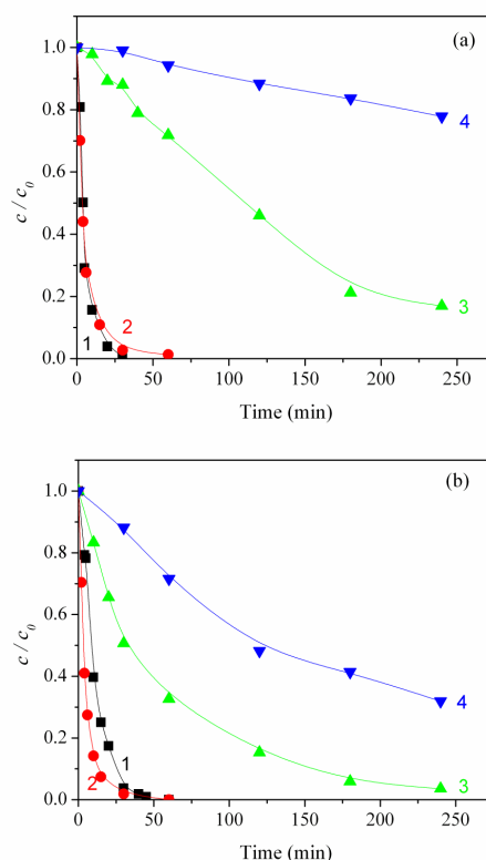
Fig. 7. Kinetics of photocatalytic degradation of MET under UV irradiation and \text{O}_2 bubbling, in the presence of \text{TiO}_2 Wackherr (a) and Degussa P25 (b): (1) MET trend, no \text{H}_2\text{O}_2 ; (2) MET trend, 3 mM \text{H}_2\text{O}_2 ; (3) TOC trend, no \text{H}_2\text{O}_2 ; (4) TOC trend, 3 mM \text{H}_2\text{O}_2 .
