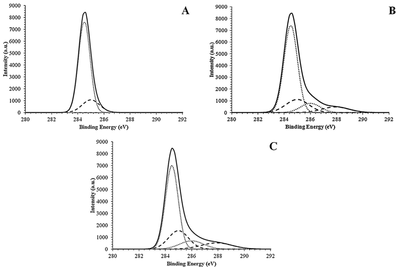
Figure 3. XPS spectra in the 280-292 eV range. Solid line curves: experimental curves; dotted lines: C-C signal at 284.5 eV and C-O signal at 286.0 eV; dashed lines: C-H signal at 285.0 eV and C=O signal at 287.9 eV. Spectra normalized at 284.5 eV. Section A: original not treated PP fibers; section B: He/O 2 plasma treated PP fibers (1050 W); section C: He/O 2 /H 2 O plasma treated PP fibers (1050 W).
