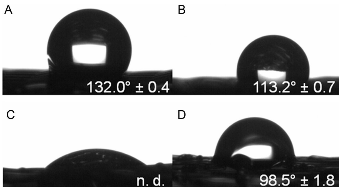
Figure 4. DSA analyses of PP fibers: (A) before plasma treatments; (B) after He plasma treatment; (C) after He/O 2 plasma treatment; (D) after He/O 2 /H 2 O plasma treatment.
