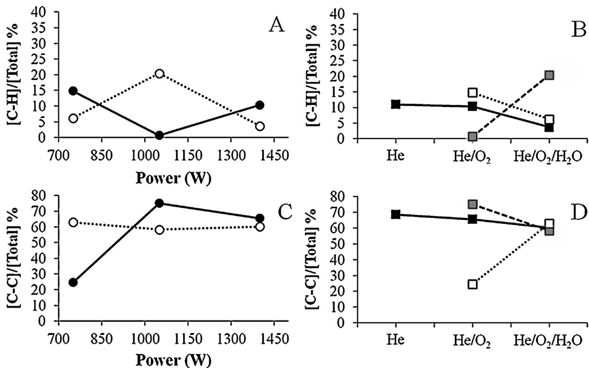
Figure 5. XPS intensities trends showing integral area of each contribution normalized in respect to the total C1s signal. (A) C-H normalized signals vs power applied (black circles: He/O 2 plasma; white circles: He/O 2 /H 2 O); (B) C-H normalized signals vs different types of plasmas (white squares: 750 W; grey squares: 1050 W; black squares: 1400 W); (C) C-C normalized signals vs power applied (black circles: He/O 2 plasma; white circles: He/O 2 /H 2 O); (D) C-C normalized signals vs different types of plasmas (white squares: 750 W; grey squares: 1050 W, black squares: 1400 W).
