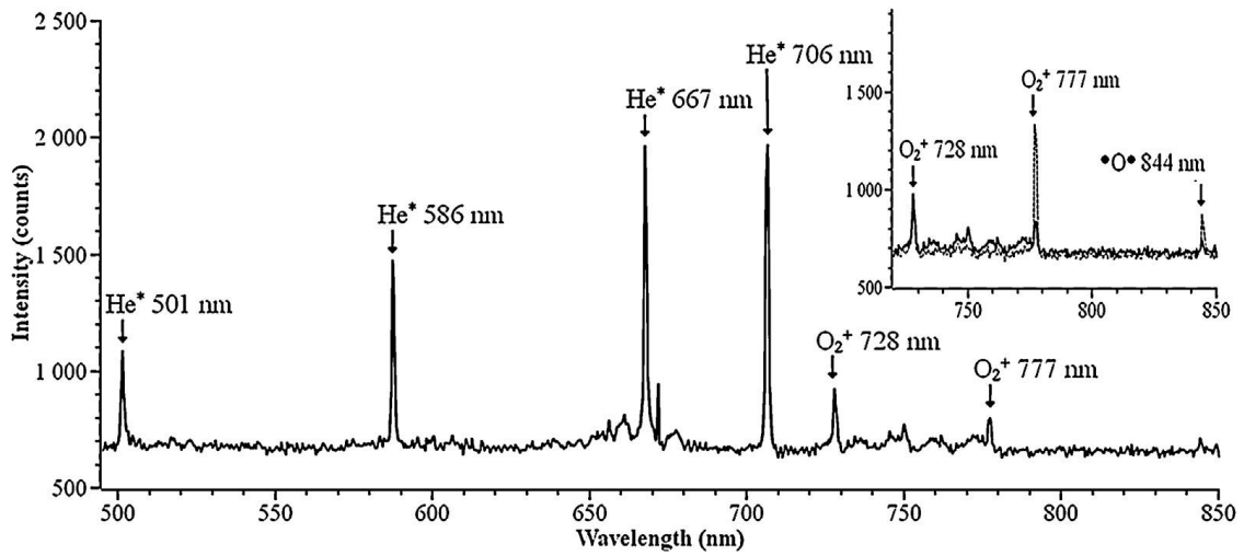
Figure 1. OES spectrum in the 495-850 nm range relative to He plasma. In the inset the same spectrum in the range 720-850 nm (solid line) is reported together with the He/O 2 plasma one (dotted line). The principal signals are labeled.
