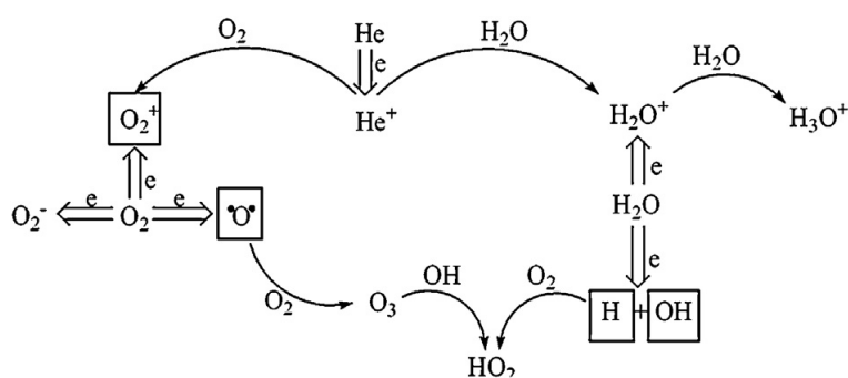
Scheme 2. He/O 2 /H 2 O plasma phase reaction pathway. The squares evidence chemical species detected by OES.
