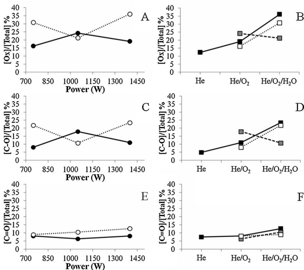
Figure 6. XPS intensities trends showing integral area of each contribution normalized in respect to the total C1s signal. (A) Oxidized species (C-O + C=O) normalized signals vs power applied (black circles: He/O 2 plasma; white circles: He/O 2 /H 2 O); (B) oxidized species (C-O + C=O) normalized signals vs different types of plasmas (white squares: 750 W; grey squares: 1050 W; black squares: 1400 W); (C) C-O normalized signals vs power applied (black circles: He/O 2 plasma; white circles: He/O 2 /H 2 O); (D) C-O normalized signals vs different types of plasmas (white squares: 750 W; grey squares: 1050 W; black squares: 1400 W); (E) C=O normalized signals vs power applied (black circles: He/O 2 plasma; white circles: He/O 2 /H 2 O); (F) C=O normalized signals vs different types of plasmas (white squares: 750 W; grey squares: 1050 W; black squares: 1400 W).
