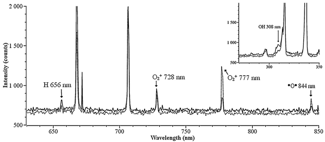
Figure 2. OES spectra in the 630-850 nm range: He/O 2 /H 2 O plasma (solid line) and He/O 2 plasma (dotted line). In the inset the same spectra in the range 270-350 nm. The principal signals are labeled.
