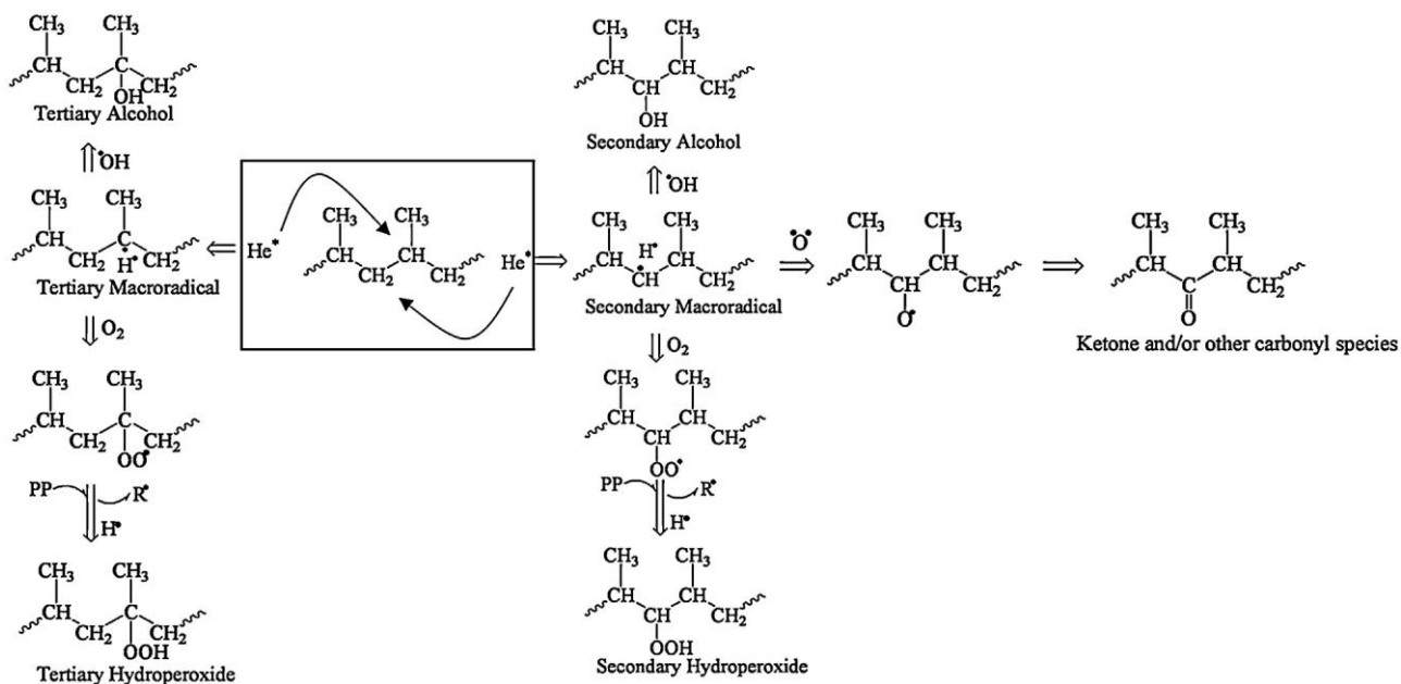
Scheme 3. He/O 2 /H 2 O plasma reaction mechanism on PP surface. The square indicates the first reaction step.
