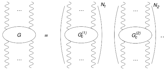
Figure 3. Decomposition of a soft photon graph into connected subdiagrams G_c^{(i)} , each of which occurs N_i times.
