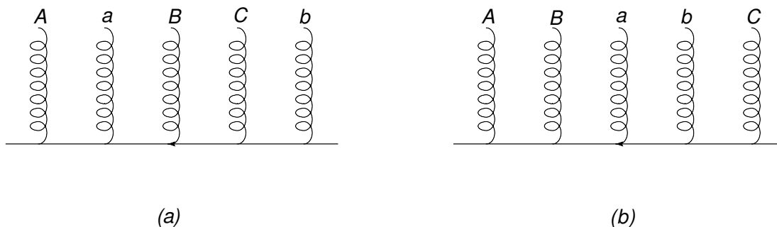
Figure 11. Simple example of two groups of gluon emissions on a single eikonal line. See the discussion in the text.
