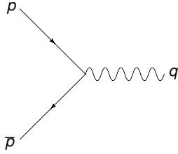
Figure 15. Born level diagram for the Drell-Yan production of a an off-shell photon.
