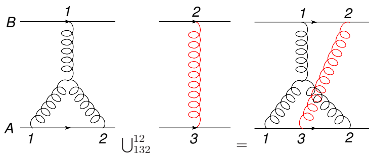
Figure 6. Illustration of the merging product \cup_{\pi_A}^{\pi_B} between two eikonal graphs, where \pi_A and \pi_B are permutations of the gluons on eikonal lines A and B such that ordering within each group is held fixed.
