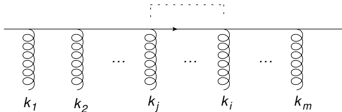
Figure 13. Schematic form of diagrams involving a two-gluon vertex. Additional eikonal emissions may occur between the two correlated gluons.
