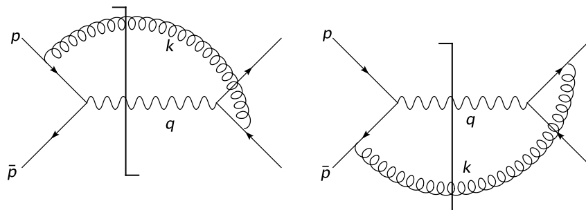
Figure 16. Squared matrix elements contributing at NLO in the eikonal limit. The cut denotes the final state.
