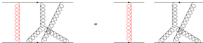
Figure 4. Decomposition of a higher order non-Abelian diagram in terms of webs.
