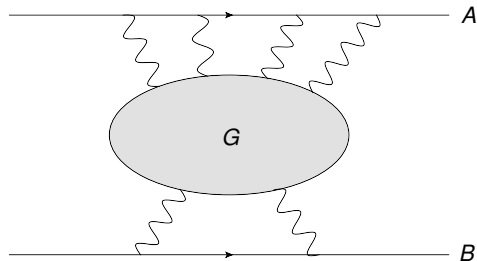
Figure 2. A process involving two eikonal lines A and B, interacting through the exchange of soft gluons forming diagram G .
