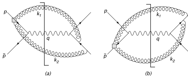
Figure 18. Cut Feynman diagrams involving the next-to-eikonal two-gluon vertices summarized by the tensor R^{\mu\nu} . Note that also the complex conjugate diagrams must be included.
