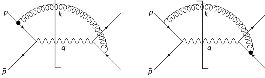
Figure 17. Diagrams contributing at NE level to the squared amplitude for NLO real emission. Two additional diagrams, arising from complex conjugation, are not shown.
