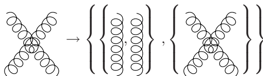
Figure 7. A diagram and its set of decompositions. The first decomposition has m_{\mathbf{I}} = 2 and m_{\mathbf{X}} = 0 , the second decomposition has m_{\mathbf{I}} = 0 and m_{\mathbf{X}} = 1 .
