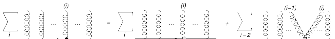
Figure 10. Schematic representation of the theorem given in eq. (3.12). Here \bullet denotes a vertex which depends upon a sum of gluon momenta, and \square a vertex depending only upon the momenta entering the chosen vertex.
