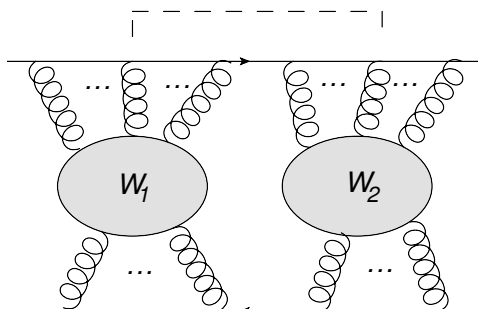
Figure 14. A diagram composed of two eikonal webs W_1 and W_2 , correlated by a next-to-eikonal two-gluon vertex. Such diagrams contribute to the NE exponent, and thus can be described as NE webs.
