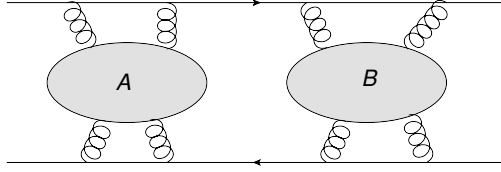
Figure 8. General form of a diagram which is two-eikonal-line reducible.
