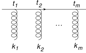
Figure 12. A series of emissions from an external line in position space. In a non-abelian theory, emissions are ordered, and path ordering of the color matrices is equivalent to time ordering of the emissions, with t_1 < t_2 < \dots < t_m .
