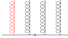
Figure 5. Gluon groups obtained from the lower eikonal line of figure 4, with the same color coding as in that figure.
