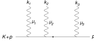
Figure 1. Soft photon emission from an energetic line.
