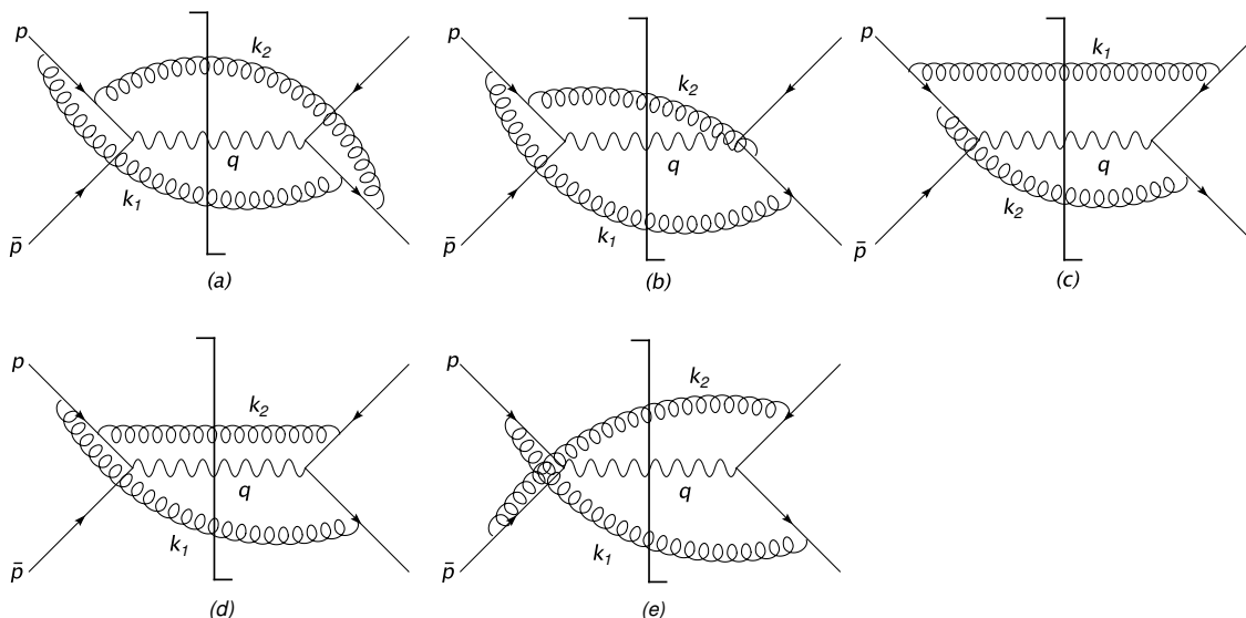
Figure 19. Diagrams for the double-real-emission contribution to the NNLO Drell-Yan K factor discussed in the text. A cut is implied over the intermediate state in each case, and complex conjugates of the above diagrams (excluding (e), which is real) must also be included.
