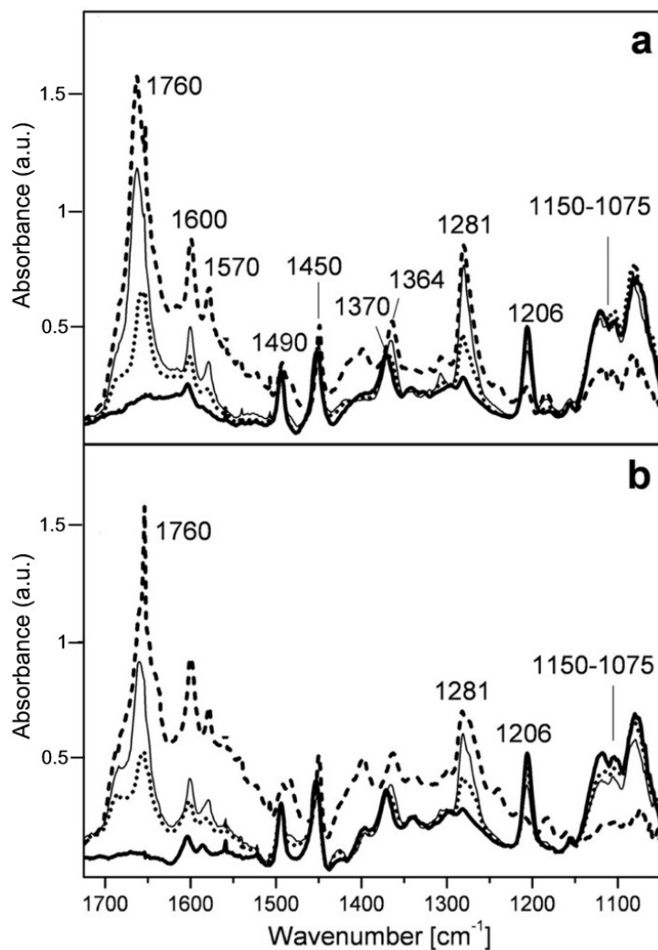
Fig. 2 FTIR spectra of 1-phenylethanol- O_2 interaction (section a) and of 1-phenylethanol/toluene- O_2 interaction (section b) on AuTiDeg surface. Solid lines: adsorbed alcohol or alcohol/toluene. Dotted lines: after O_2 inlet. Fine line: after 30' of O_2 interaction. Dashed lines: mixture heated at 80 °C (section a) and at 110 °C (section b).
