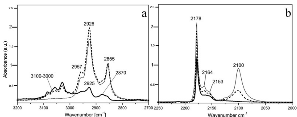
Fig. 4 Section a: FTIR spectra of toluene adsorbed on AuTiDeg at r.t. (bold curve), heated at 110 °C (dotted curve) and outgassed 30' at r.t. (fine curve). Section b: FTIR spectra of CO adsorbed at -153 °C on AuTiDeg before the interaction with toluene (fine curve), after the interaction with the solvent at r.t. (dotted curve) and after heating in toluene at 110 °C (bold curve).
