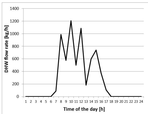
Fig. 3a. Daily load profile for DHW
