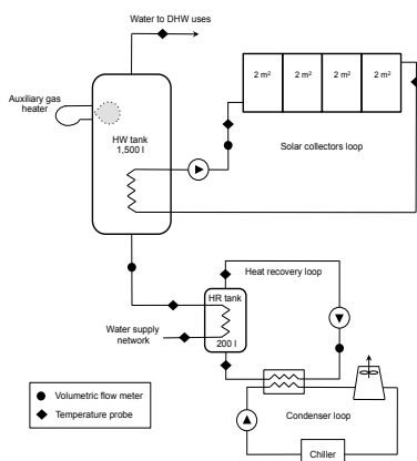
Fig. 1. Energy system scheme
