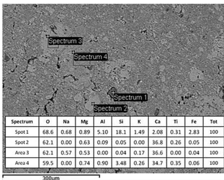
Figure 2. A SEM–BS image and EDX analyses (polished section) on sample P48. Spot 1, ceramic inclusion; Spot 2 and Area 3, calcite aggregates; Area 4, binder (marly carbonate).
