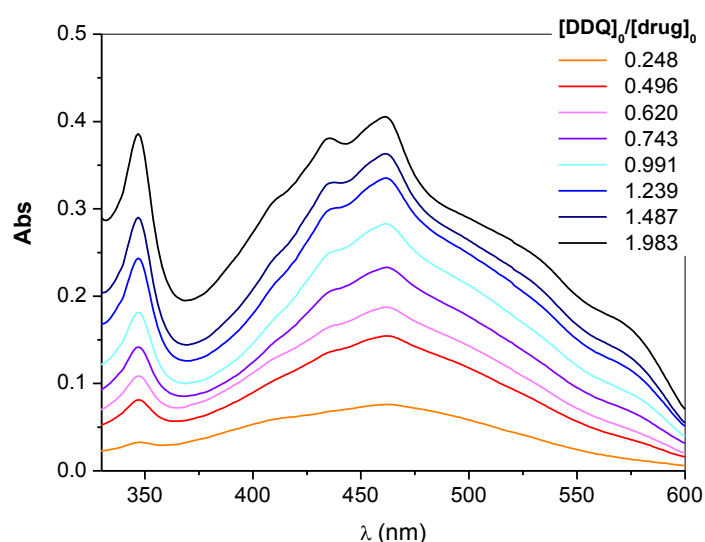
Figure 5. UV-vis spectra recorded on solutions containing different molar ratios of DDQ and atenolol in ethanol, with [drug]_0 = 3.9 \cdot 10^{-5} \text{ mol L}^{-1} and optical path 5.0 cm.
