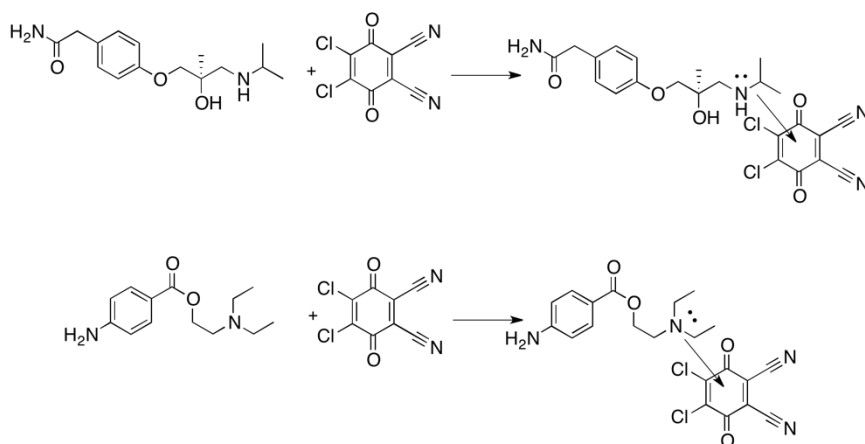
Figura 10. Molecular structures of compounds and their correspondent charge transfer complexes.
