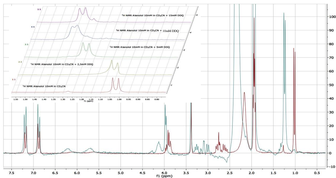
Figure 9. ^1\text{H} -NMR spectra of the drug in acetonitrile- \text{d}_3 , before and after the addition of 0.5 eq of DDQ: Atenolol 10.0 \text{ mmol L}^{-1} (red), Atenolol 10.0 \text{ mmol L}^{-1} and DDQ 5.0 \text{ mmol L}^{-1} (blue); nested graph: ^1\text{H} -NMR \text{CH}_3 -region shift observed during titration.
