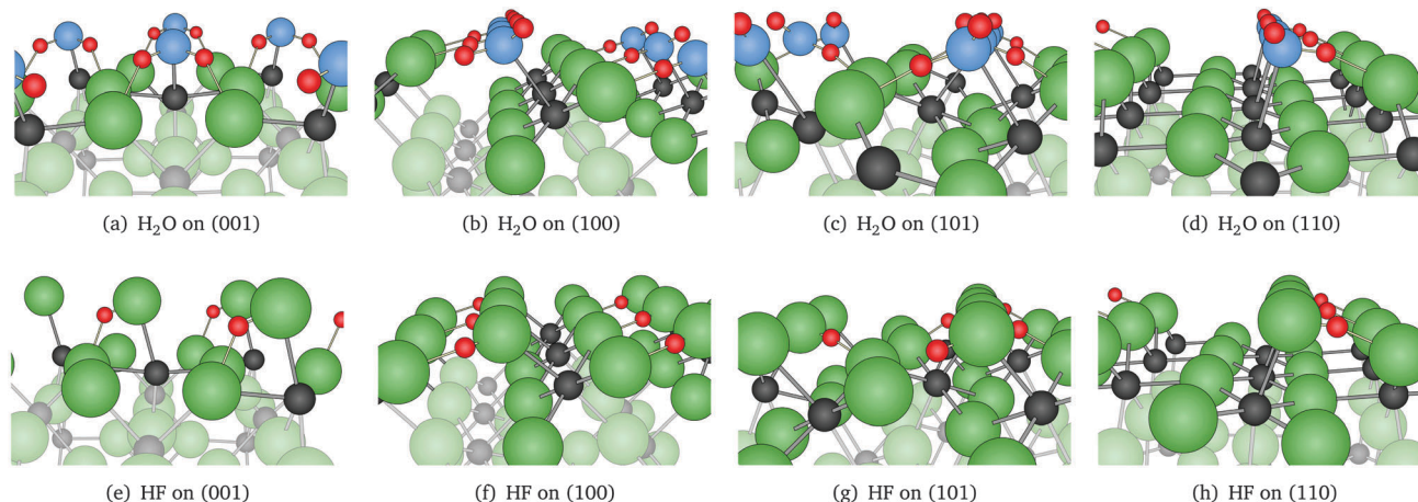
Fig. 1 Adsorption structures of H 2 O and HF on low index MgF 2 surfaces, full coverage, obtained using B3LYP. Fluorine atoms are represented as green, magnesium as black, hydrogen as red and oxygen as blue spheres. Surface atoms are highlighted.
