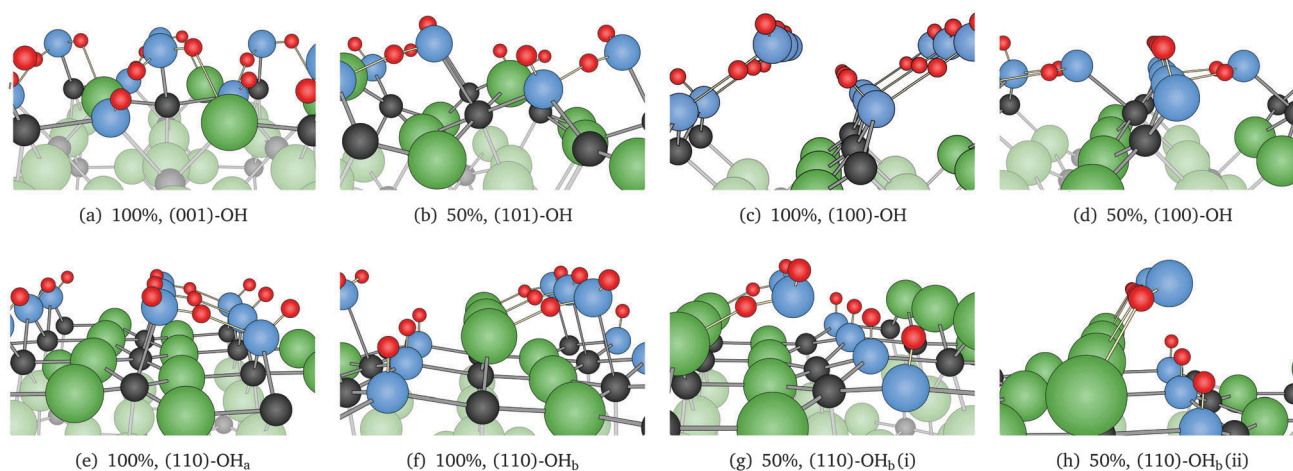
Fig. 2 Adsorption structures of H 2 O on partially hydroxylated MgF 2 surfaces obtained using B3LYP. Fluorine atoms are represented as green, magnesium as black and hydrogen as red and oxygen as blue spheres. Surface atoms are highlighted.
