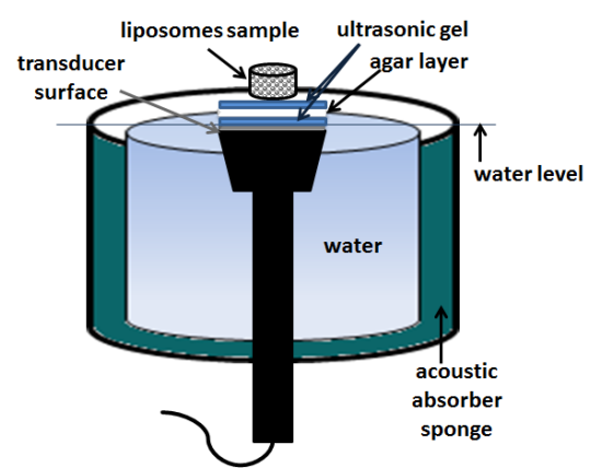
Insonation setup for in vitro experiments.
