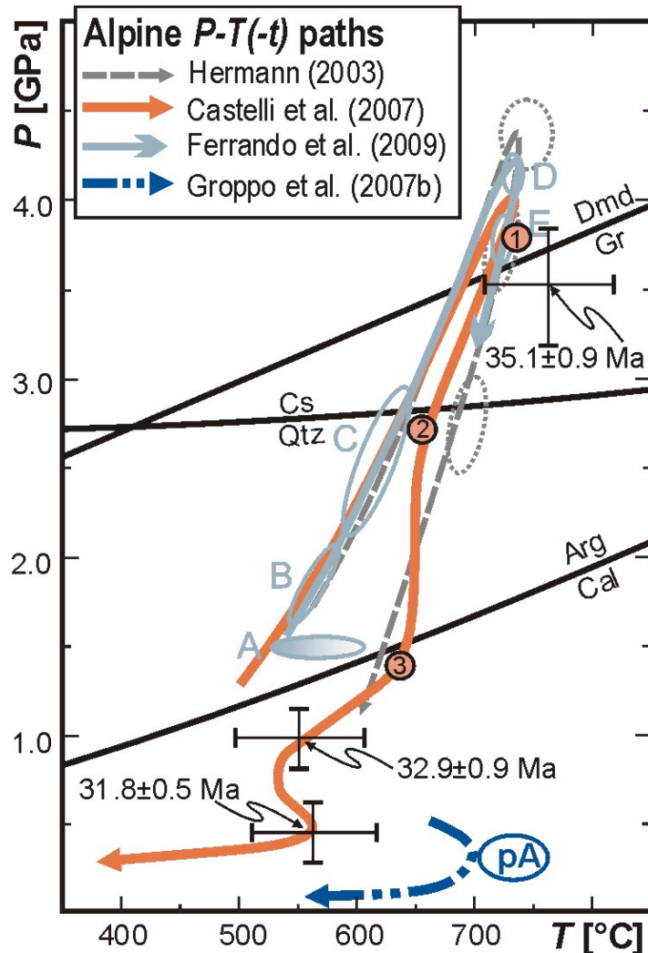
Fig. 17 - Synopsis of selected Alpine P-T estimates and inferred Alpine and pre-Alpine (blue curve: pA) P-T paths for the BIU Polymetamorphic Complex (modified from Castelli et al., 2007). The solid, orange curve is the Alpine P-T path proposed by Castelli et al. (2007) that integrates the peak and retrograde P-T estimates by Groppo et al. (2007b: circles labelled 1 to 3). Solid ellipses labelled A to E are the P-T conditions of prograde, peak and retrograde stages of the BIU, respectively, estimated by Ferrando et al. (2009), whereas dotted ellipses are those estimated by Hermann (2003). The error bars of ages refer to the geochronologically dated P-T estimates of Rubatto & Hermann (2001). The dotted-dashed blue path (pA) is the pre-Alpine P-T path of the BIU from Groppo et al. (2007a).
