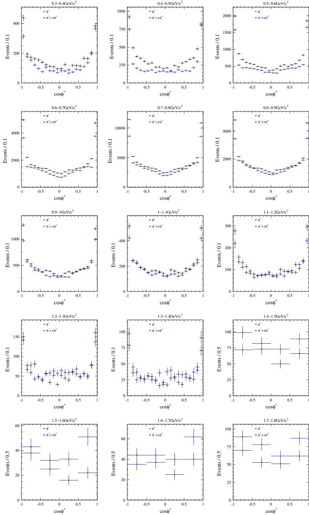
FIG. 7 (color online). The \cos\phi^* distributions for e^+e^- \rightarrow \pi^+\pi^-\gamma data in 0.1 \text{ GeV}/c^2 m_{\pi\pi} intervals. The points labeled “ \pi^- ” refer to the configurations with \phi_-^* \in [0, \pi] , while the points labeled “ \pi^- \leftrightarrow \pi^+ ” correspond to \phi_+^* \in [0, \pi] .
