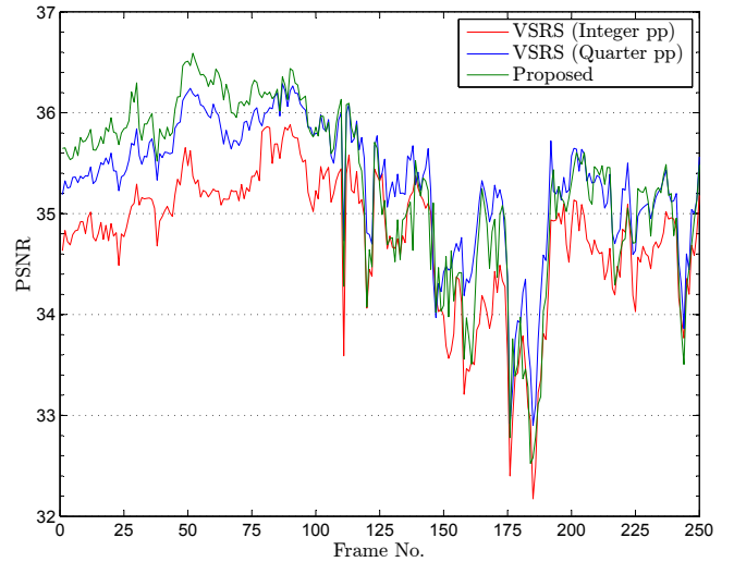
Fig. 4: Kendo sequence: PSNR comparison of the proposed technique with that of VSRS
