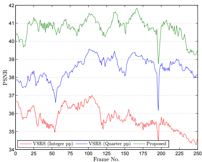
Fig. 3: Undo_Dancer sequence: PSNR comparison of the proposed technique with that of VSRS.
