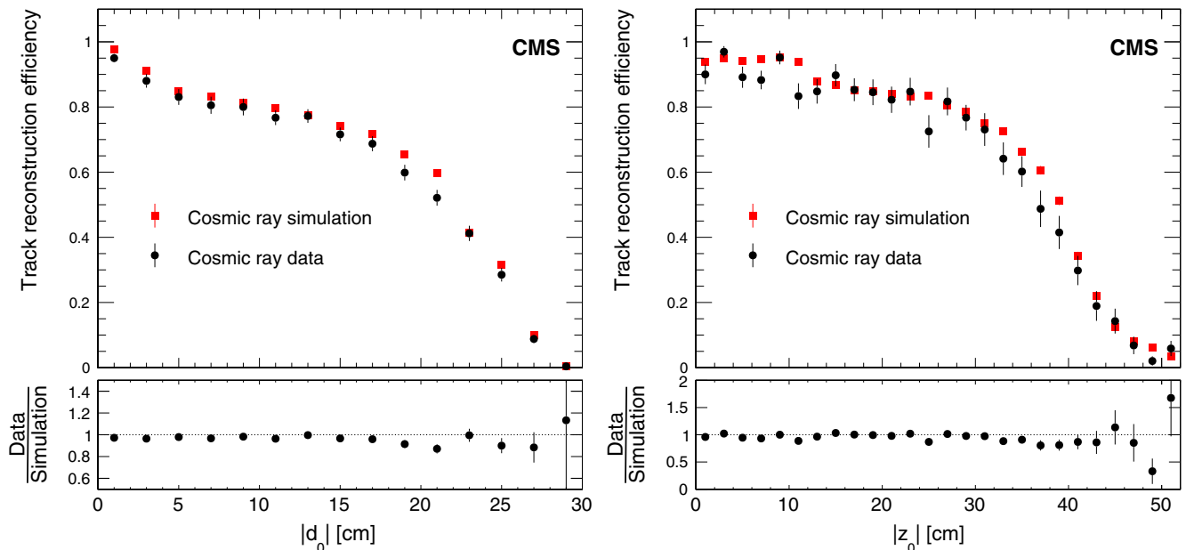
FIG. 3 (color online). Efficiency to find a track in the tracker, measured using cosmic ray muons reconstructed in the muon detectors, as a function of the transverse (left) and longitudinal (right) impact parameters (relative to the nominal interaction point of CMS). The efficiency is plotted in bins of 2 cm width. For the left plot, the longitudinal impact parameter |z_0| is required to be less than 10 cm, and for the right plot, the transverse impact parameter |d_0| must be less than 4 cm. The bottom panels show the ratio of the efficiency in data to that in simulation. The uncertainties in the simulation are smaller than the size of the markers and are not visible.
