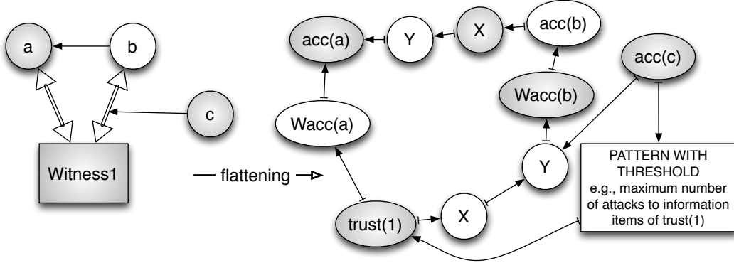
Figure 7: Feedback between the information items and sources.
