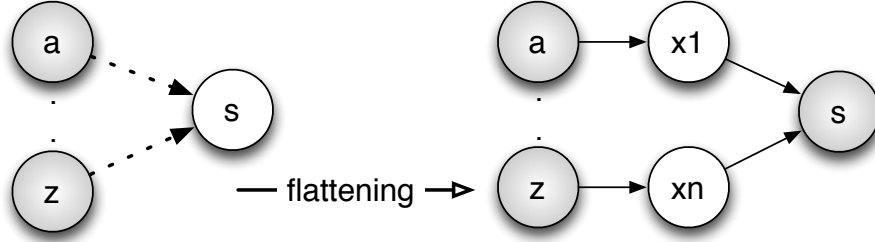
Figure 8: The activation pattern with a threshold of n arguments.
