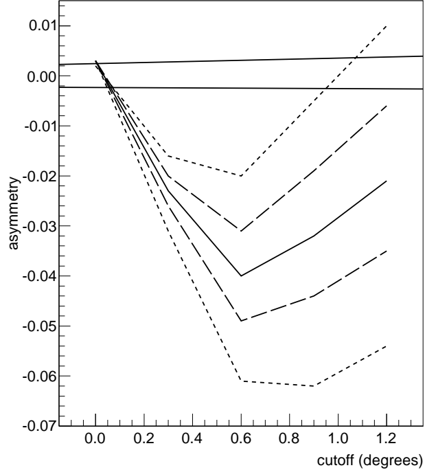
Fig. 14. Dependence of the overall (fake plus real) \cos(2\phi) -asymmetry on the cutoff angle, for different values of A_{true-\phi} , that is the real \sin(2\theta)\cos(\phi) -asymmetry integrated over all the phase space, in high energy configuration. Continuous line: A_{true-\phi} = 0 . Long-dashed lines: A_{true-\phi} = \pm 0.1 . Short-dashed lines: A_{true-\phi} = \pm 0.22 . Going from negative to positive A_{true-\phi} , the reported curves become more negative. The continuous almost horizontal lines show the \pm\sigma error band. These points have been extracted via Method 2.
