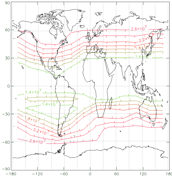
Figure 6. UV at the top of the atmosphere for albedo 100%. For albedo 0% UV light in 300-400nm (number of photons in (\text{m}^2 \text{ s})^{-1} ) will have half values. Map is in geographic coordinates.
