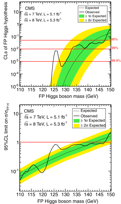
Fig. 6. (Top) The observed and expected CL_s values for the FP Higgs boson hypothesis as a function of the Higgs boson mass in the range 110–150 GeV. (Bottom) The observed and expected 95% CL upper limits on the signal strength modifier, \mu = \sigma/\sigma_{FPH} , as a function of the FP Higgs boson mass in the range 110–150 GeV.
