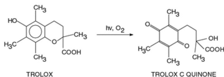
Scheme 1 Reaction of photooxidation of Trolox
