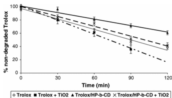
Fig. 5 Time evolution of Trolox ( 1.0 \times 10^{-3} M) in HEC gel, pure and complexed with HP- \beta -CD, in the absence and in the presence of TiO 2 , at pH 3.8
