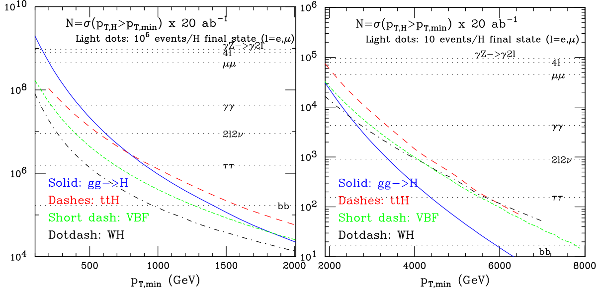
Fig. 40: Integrated Higgs transverse momentum rates, for various production channels, with 20 \text{ ab}^{-1} . The light-dotted horizontal lines in the left (right) panel correspond to the production of 10^5 ( 10 ) events with a Higgs decay to the indicated final states.
