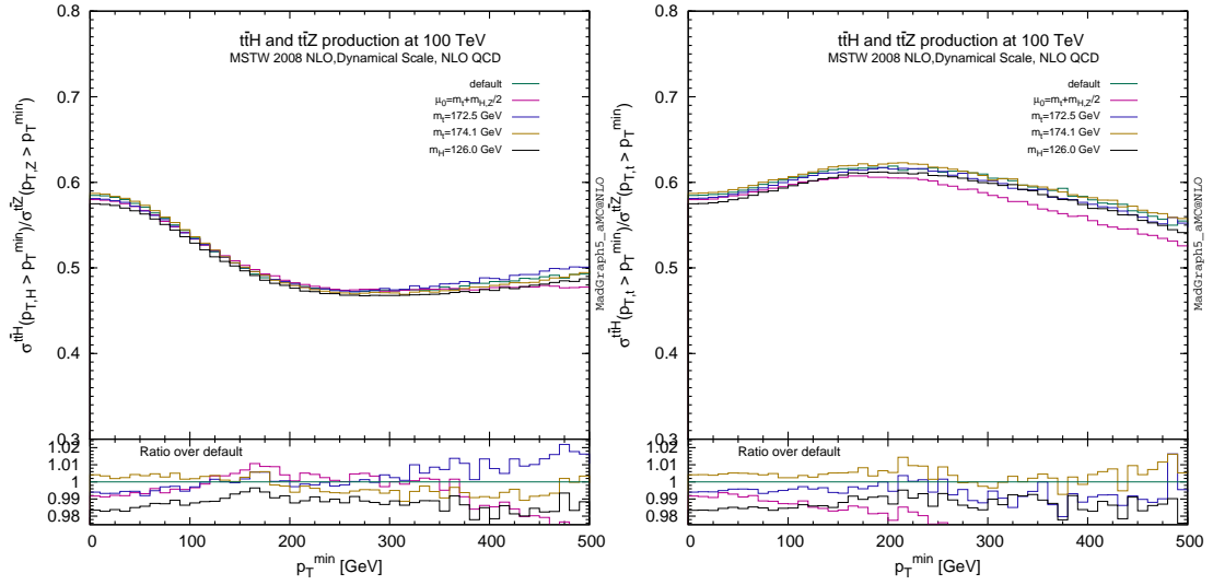
Fig. 38: Other systematics of ratios of integrated p_T spectra for different observables, at 100 TeV. From left to right: p_T of the boson, p_T of the top quark.
