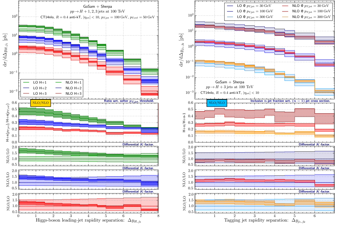
Fig. 14: The rapidity separation \Delta y_{H,j_1} between the Higgs boson and the hardest jet in H+1, 2, 3-jet production and the rapidity separation \Delta y_{j_1,j_2} between the two hardest jets in H+3-jet production at a 100 TeV proton–proton collider. The spectra for the latter are shown for varying jet- p_T thresholds. Again, the layout of the left and the right plot corresponds to the layout employed in Figure 11 and 12, respectively.
