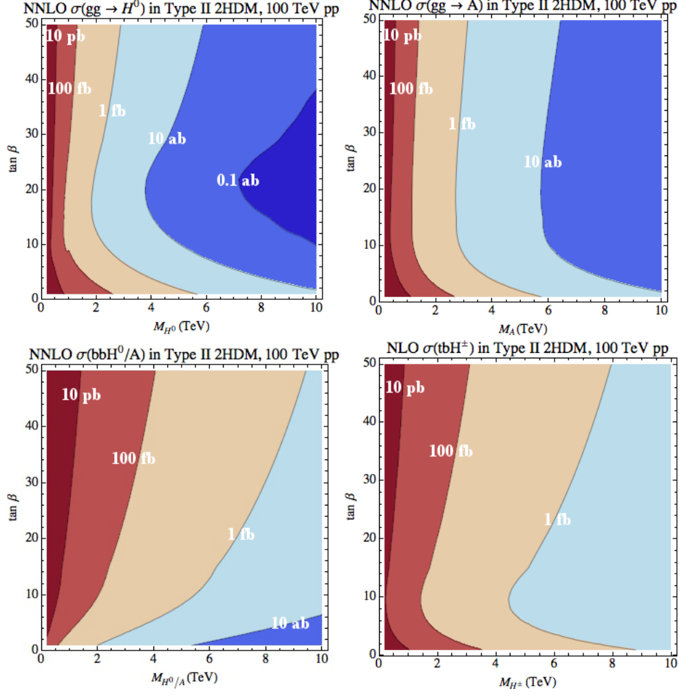
Fig. 87: Dominant production cross sections for non-SM like Higgses in the Type II 2HDM at the 100 TeV pp collider: NNLO cross section for gg \rightarrow H^0 or A (top left and top right panel, calculated using HIGLU [504] with the NNPDF2.3 parton distribution functions [125]), NNLO cross section for bottom-associated production bbH^0/A (lower left panel, calculated using SusHi [407, 505, 506]. bbH^0 and bbA cross sections are the same in the alignment limit), NLO cross section for tbH^\pm (lower right panel, calculated in Prospino [507, 508]).
