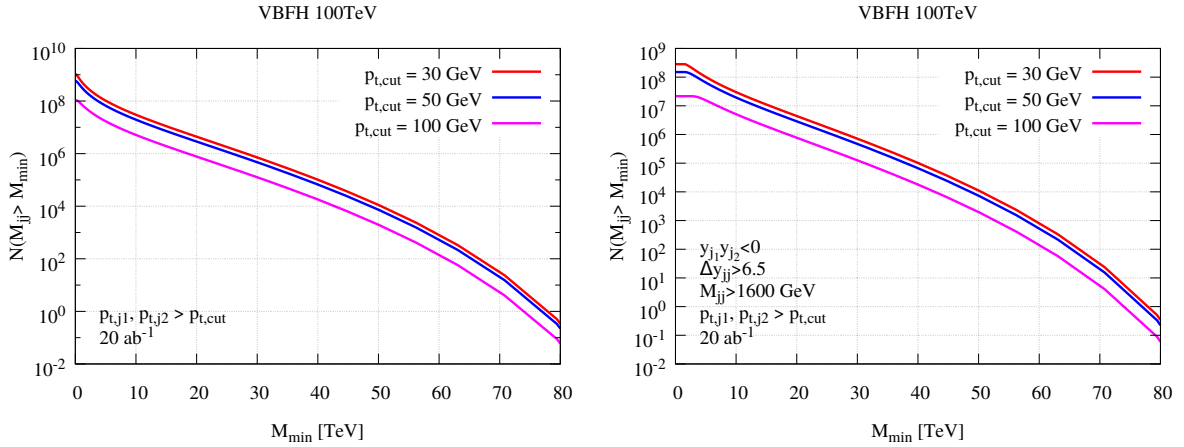
Fig. 31: The total number of VBFH events produced with M_{j_1 j_2} > M_{min} at a 100 TeV collider with an integrated luminosity of 20 \text{ ab}^{-1} . Left panel: Three different jet p_t cuts applied but no VBF cuts applied. Right panel: VBF cuts of eq. (18) and three different jet p_t cuts applied.
