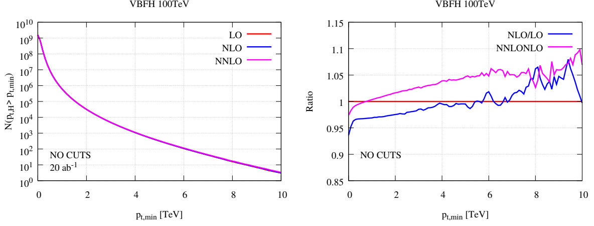
Fig. 30: The total number of VBFH events produced with p_{t,H} > p_{t,min} at a 100 TeV collider with an integrated luminosity of 20 \text{ ab}^{-1} with no cuts applied. Left panel: Spectrum computed at LO, NLO and NNLO in QCD. Due to the small corrections the difference between the three curves is hard to see by eye. Right panel: The k-factor going from LO to NLO and NLO to NNLO.
