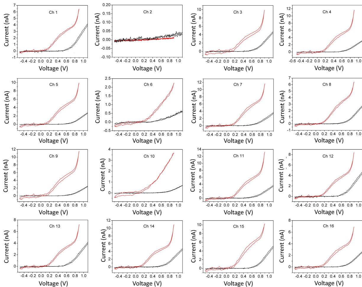
Figure 3. Cyclic voltammery characterization. Cyclic voltammetric scans at 20 \text{ mV s}^{-1} rate of a -0.5 \div 1.1 \text{ V} ramp voltage applied to all microelectrodes with respect to the quasi-reference Ag/AgCl electrode in the presence of Tyrode buffer (solid black lines) and 100 mM adrenaline solution (solid red lines). All electrodes show the characteristic features of water oxidation at a voltage higher then +0.850 \text{ V} , while detecting the oxidation of adrenaline at voltages between +500 \text{ mV} and +800 \text{ mV} , with the exception of electrode #2.
