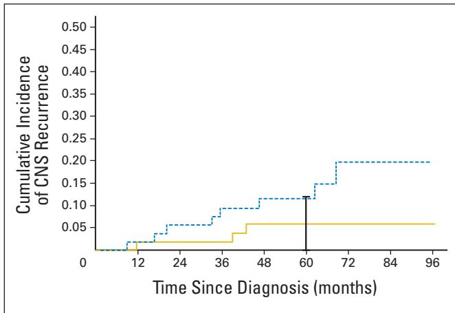
Fig 4. Cumulative incidence of CNS recurrence (solid gold line) and cumulative mortality without CNS involvement (dashed blue line); 5-year CNS cumulative incidence, 5.9% (95% CI, 0% to 12%). Vertical bar represents 95% CI.
