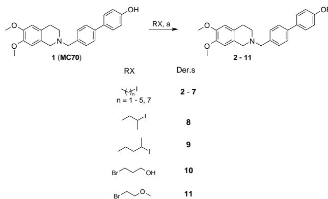
Scheme 1. Reagents and conditions. a) \text{K}_2\text{CO}_3 , \text{CH}_3\text{CN} , reflux.
