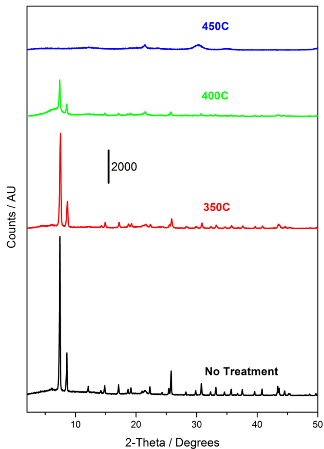
Figure S52: PXR D patterns recorded on UiO-66-160-2:1-MeOH after 12 hour exposures (in air) to the temperatures indicated on the figure. Monoclinic \text{ZrO}_2 begins to form after treatment at 450 °C, as evidenced by the emergence of broad and low intensity reflections at 30.3 and 35.1 2 \theta .
