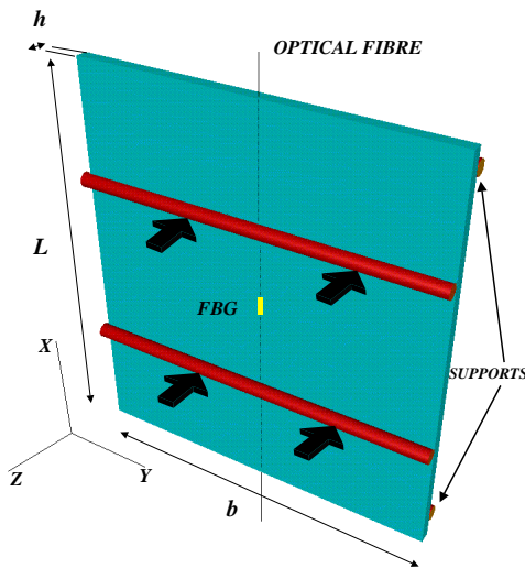
Fig. 1. Geometry of a specimen subjected to 4-point bending.
